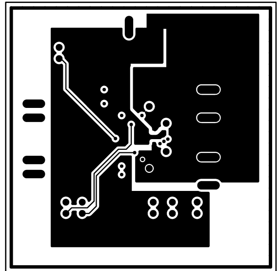
Top Soldermask
