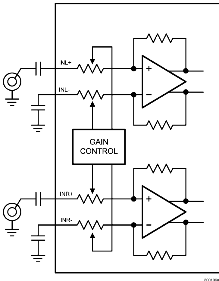
FIGURE 2. Single-Ended Circuit Diagram
