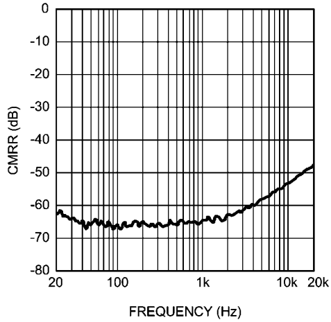
CMRR vs Frequency V_{DD} = 3.6V , V_{CM} = 1V_{P-P} , R_L = 8\Omega
