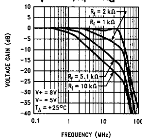
Frequency Response vs R_F
