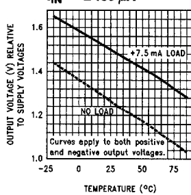
V_{OUT} Referred to Supplies
