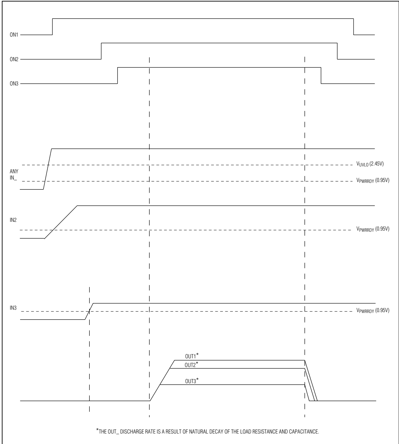
Figure 2. Voltage-Tracking Timing Diagram (Provided t_D , V_{UVLO} Requirement is Met)
