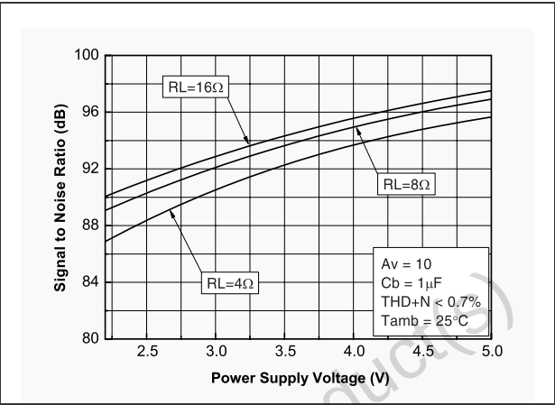
Figure 57. Signal to noise ratio vs. power supply with unweighted filter (20Hz to 20kHz)
