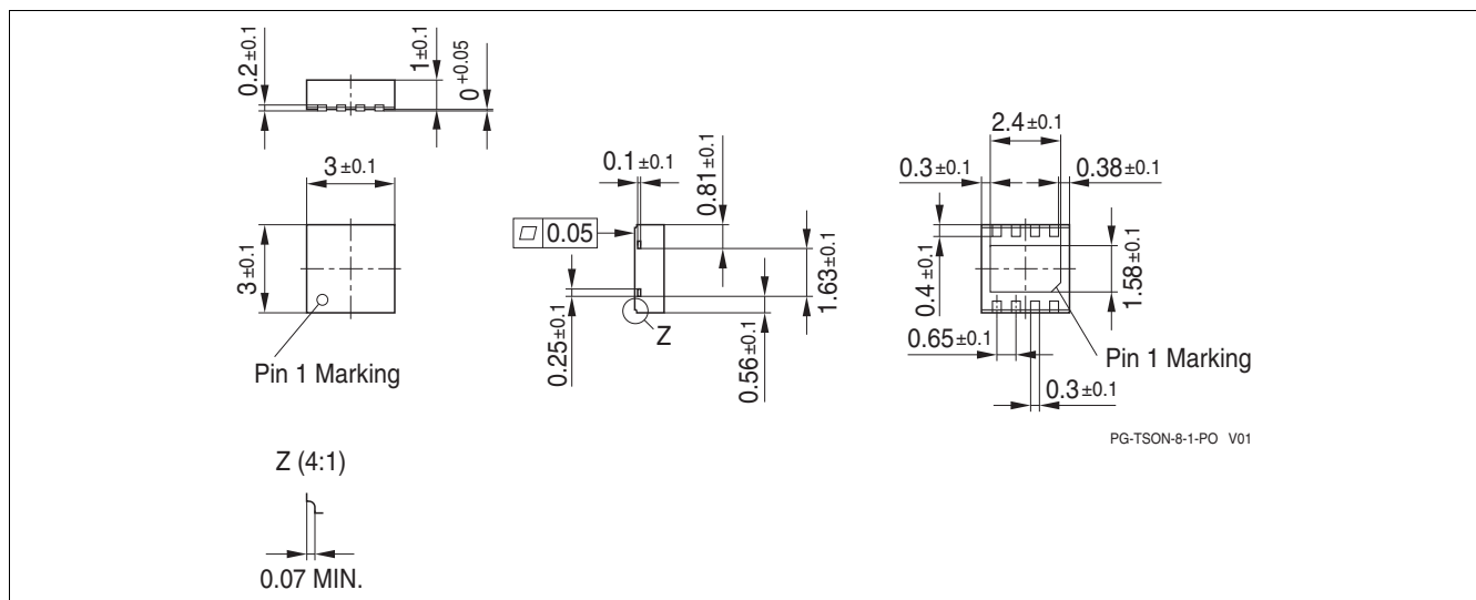
Figure 20 PG-TSON-8 (Plastic thin small outline nonleaded PG-TSON-8) 1)
