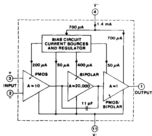
Figure 1 - Block diagram of 1/4 of the CA3410E.
