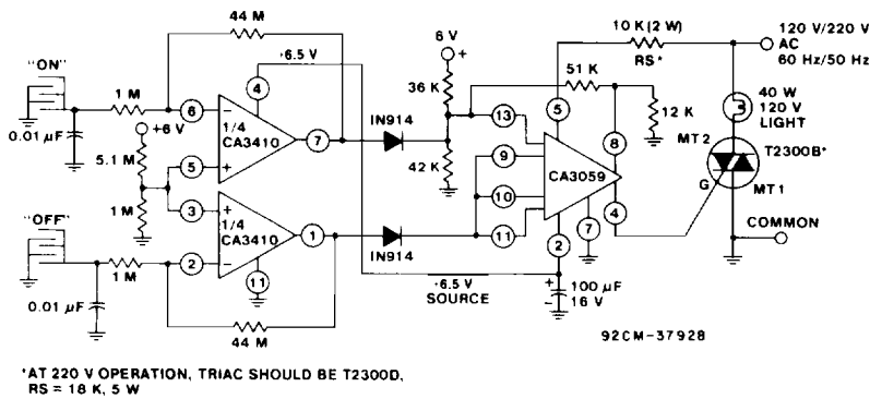
Fig. 18 - On/off touch switch.
