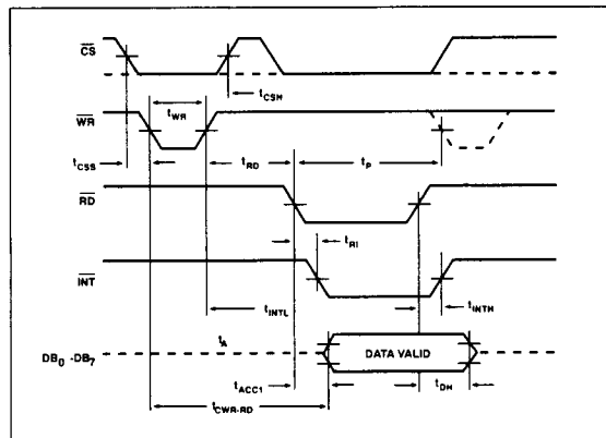
Figure 3: WR-RD Mode (Pin 7 = +5V, t_{RD} < t_{INTL} )
