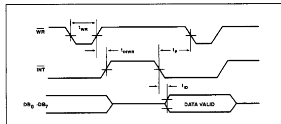
Figure 4: WR-RD Mode – Stand-Alone Operation (Pin 7 = +5V, CS = RD = 0V )
