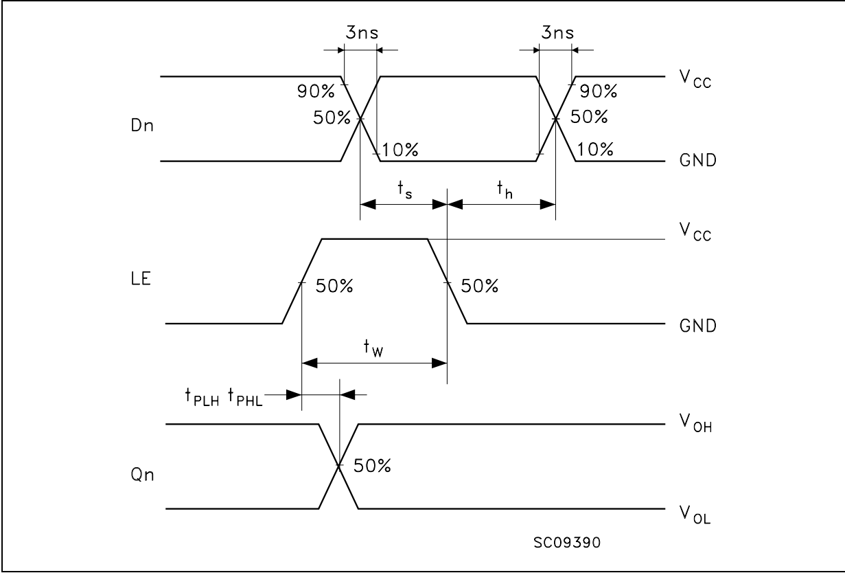
WAVEFORM 1: LE TO Qn PROPAGATION DELAYS, LE MINIMUN PULSE WIDTH, Dn TO LE SETUP AND HOLD TIMES (f=1MHz; 50% duty cycle)
