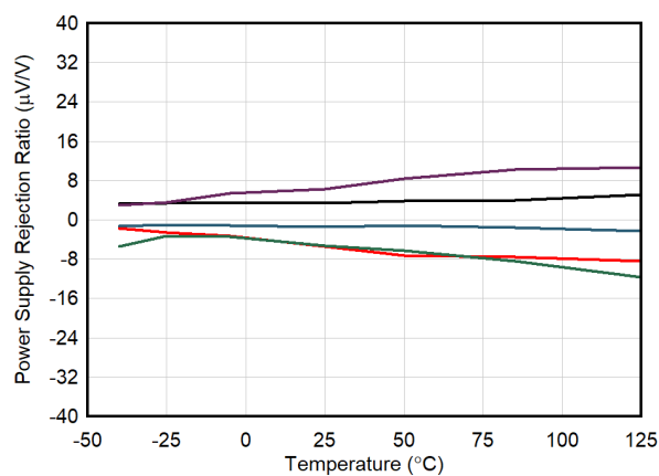
Figure 6-15. PSRR vs Temperature
