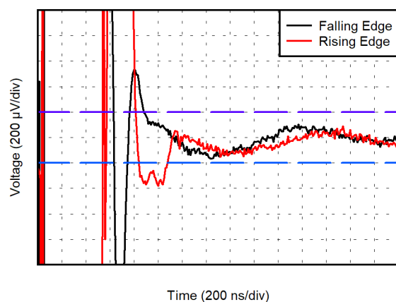
Figure 6-33. Settling Time
