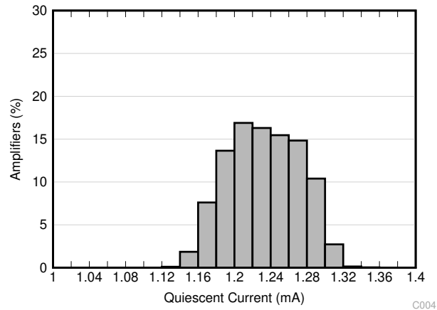
Figure 6-2. Quiescent Current Distribution
