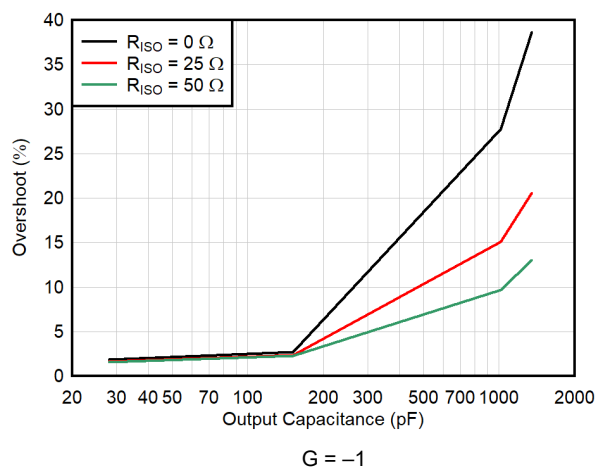
Figure 6-24. Small-Signal Overshoot vs Capacitive Load (10-mV Step)
