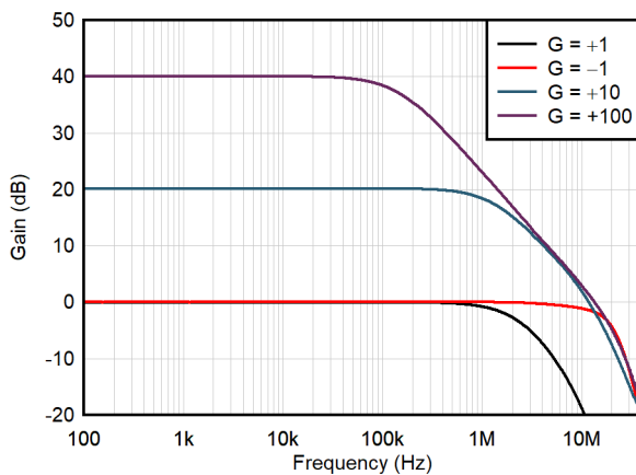
Figure 6-5. Closed-Loop Gain and Phase vs Frequency
