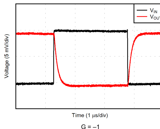
Figure 6-30. Small-Signal Step Response (10-mV Step)
