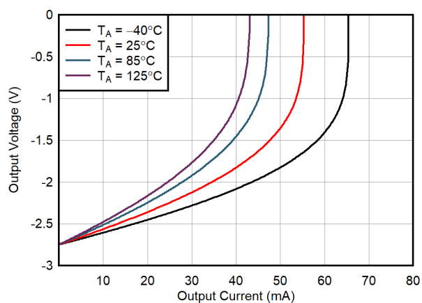
Figure 6-10. Output Voltage Swing vs Output Current (Sinking)
