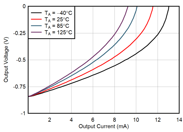
Figure 6-12. Output Voltage Swing vs Output Current (Sinking)
