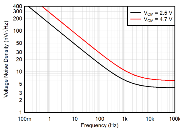
Figure 6-16. Voltage Noise vs Frequency
