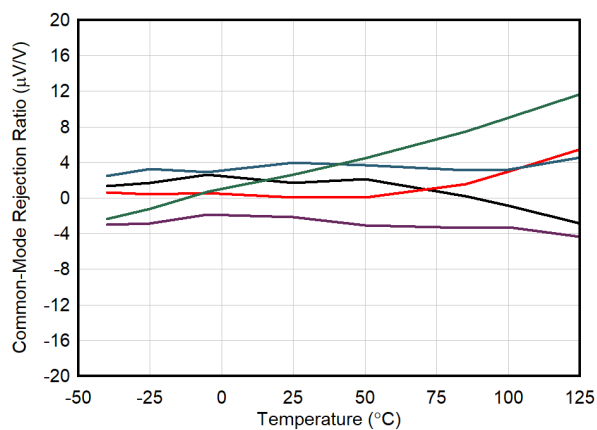
Figure 6-14. CMRR vs Temperature
