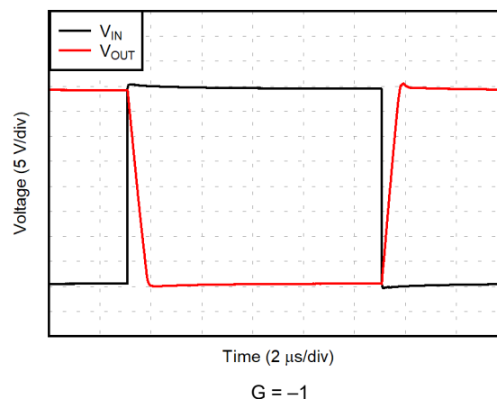
Figure 6-32. Large-Signal Step Response (4-V Step)
