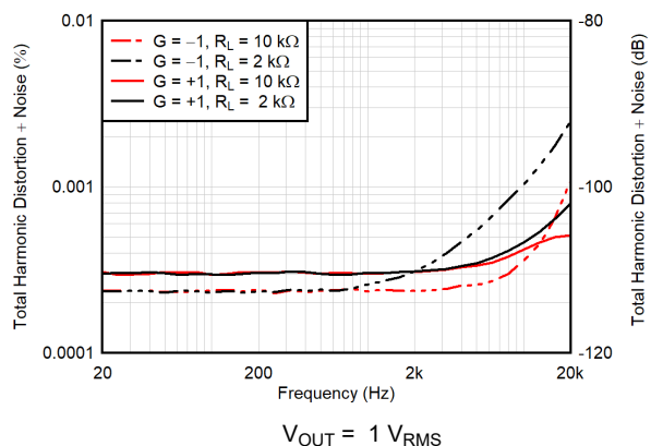
Figure 6-17. THD+N Ratio vs Frequency
