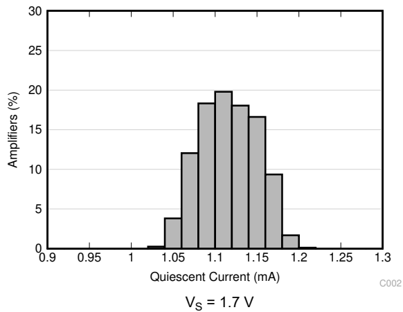
Figure 6-3. Quiescent Current Distribution
