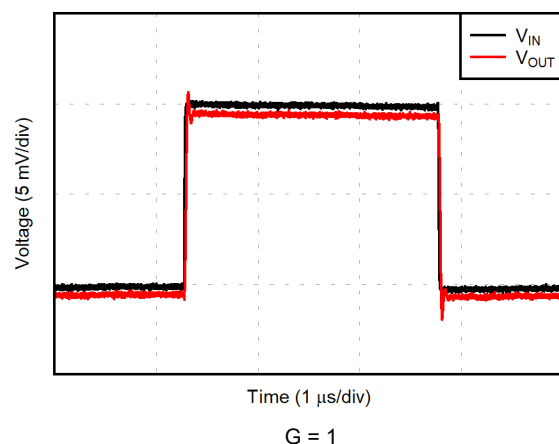
Figure 6-29. Small-Signal Step Response (10-mV Step)
