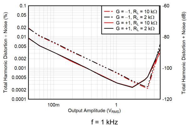
Figure 6-18. THD+N vs Output Amplitude
