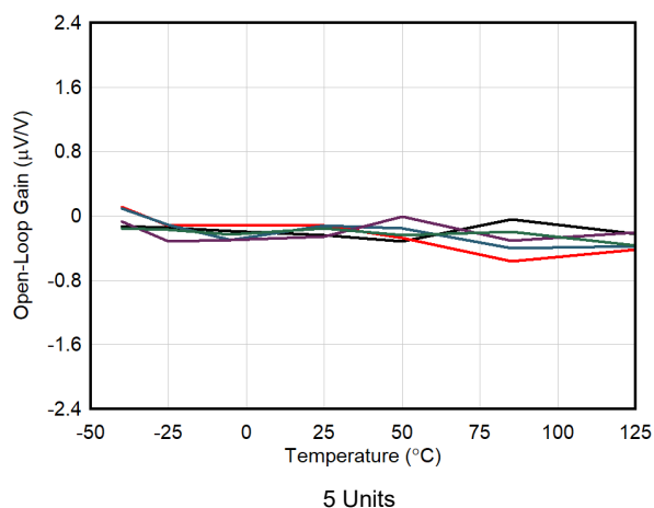
Figure 6-22. Open-Loop Gain vs Temperature
