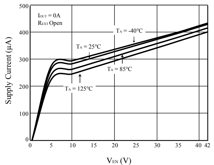
Figure 13 I_{EN} vs. V_{EN}
