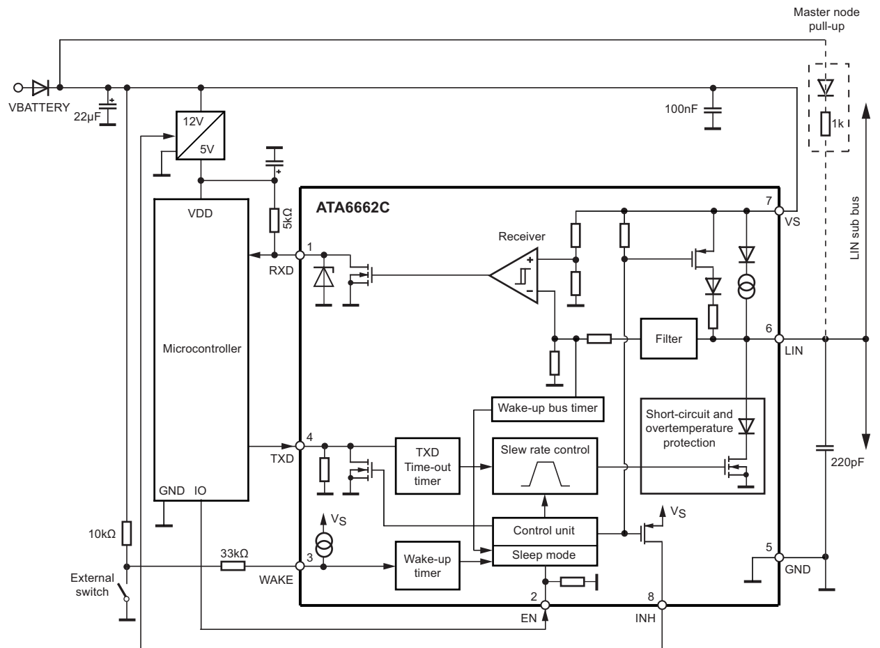
Figure 6-2. Application Circuit
