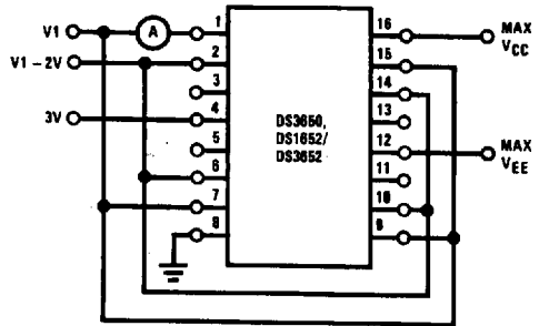
FIGURE 5. I_{iH}
