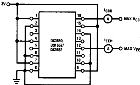
FIGURE 2. I CC and I EEH
