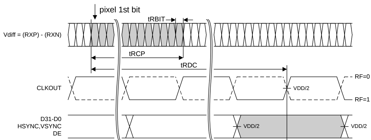
Figure 26. THCV236 Latency
