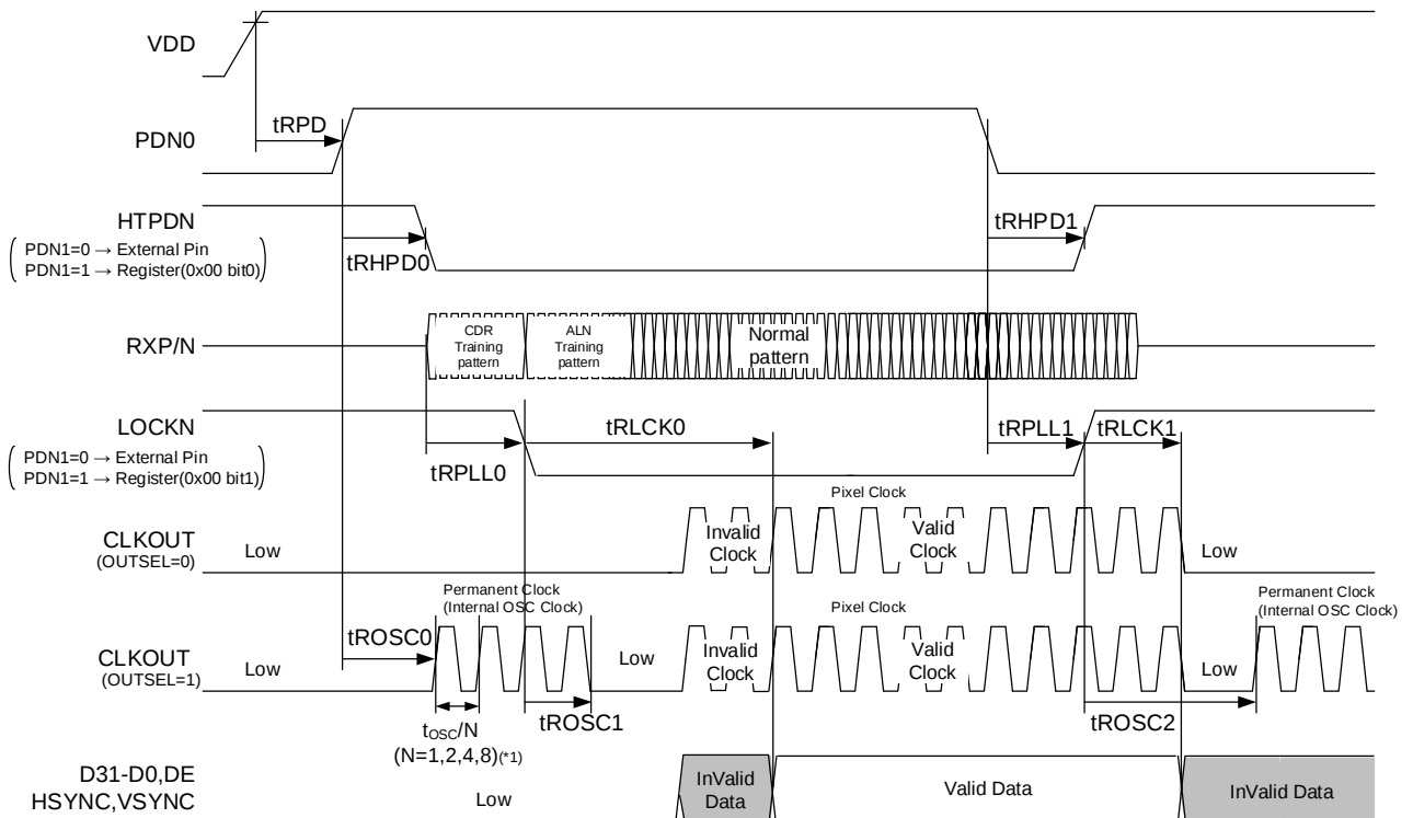
Figure 27. THCV235 Lock/Unlock Sequence
