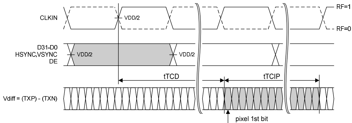
Figure 25. THCV235 Latency
