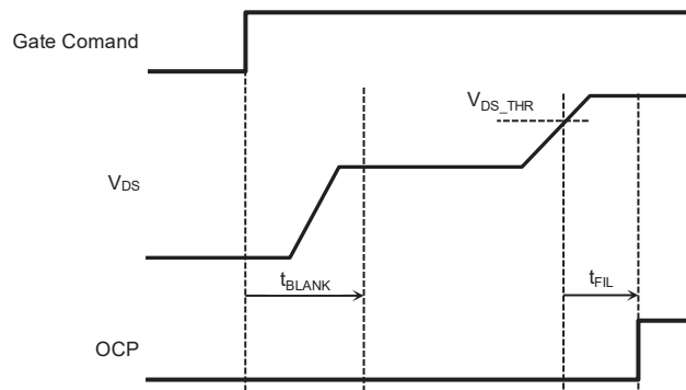
Figure 5: OCP timing diagram
