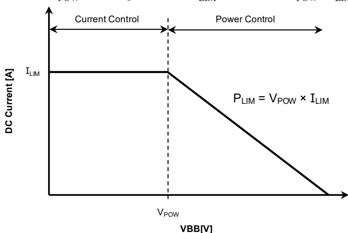
Figure 2 : Power Limit
