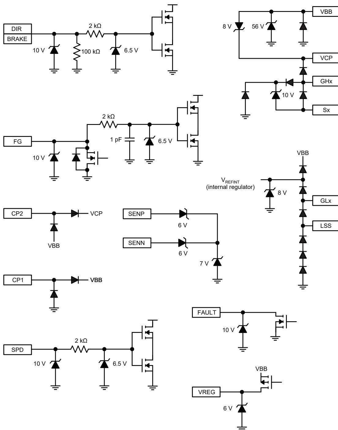
Figure 8: Terminal Diagrams
