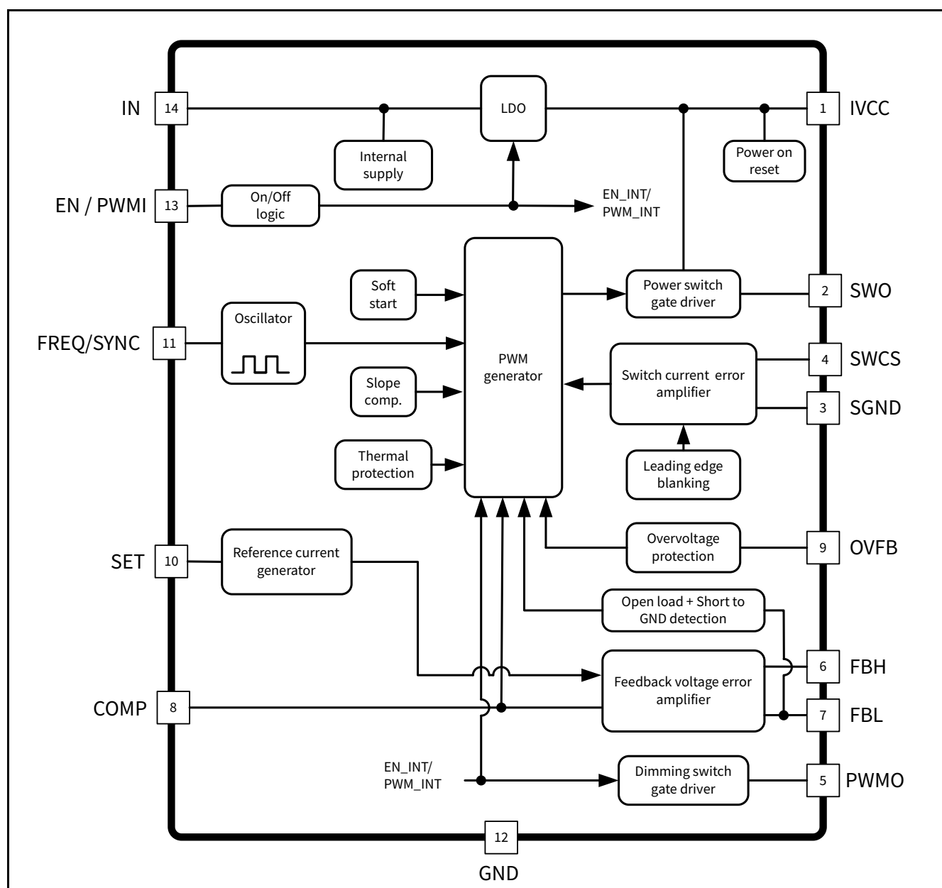
Figure 2 Block diagram TLD5098EP
