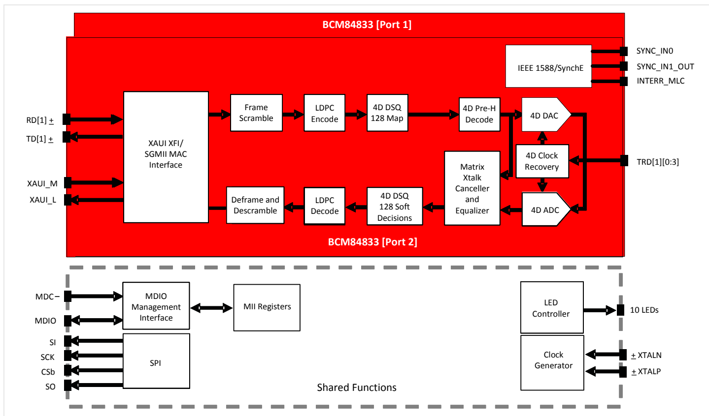
BCM84833 Block Diagram for Each Port
