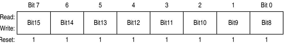
Figure 15-7. TIM Counter Modulo High Register (TMODH)
