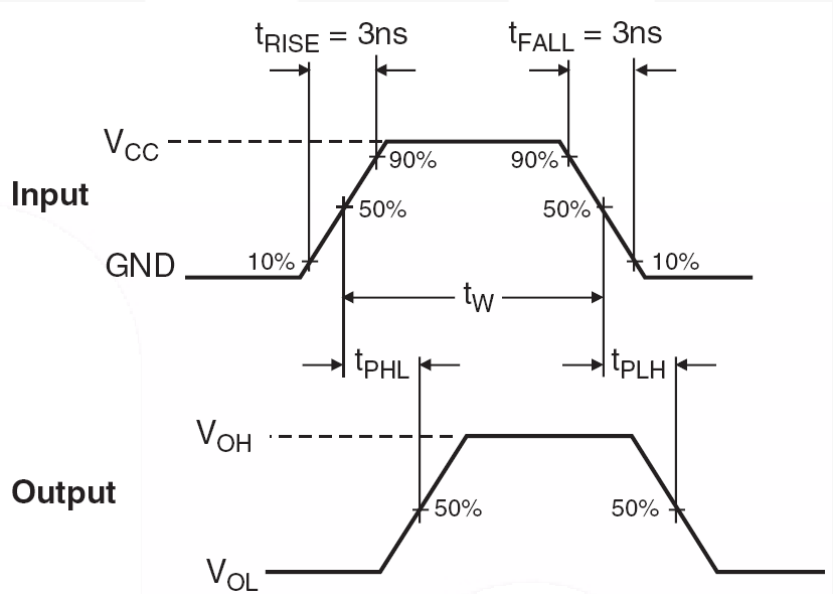
Figure 6. AC Waveforms
