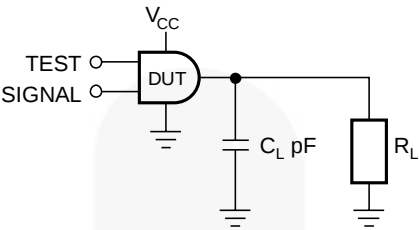
Figure 5. AC Test Circuit
