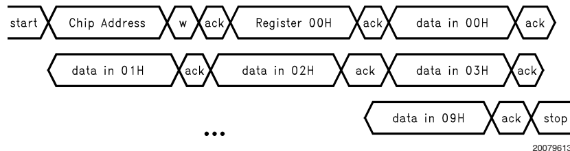
FIGURE 8. Programming with Auto Increment Enabled (in WRITE Mode)
