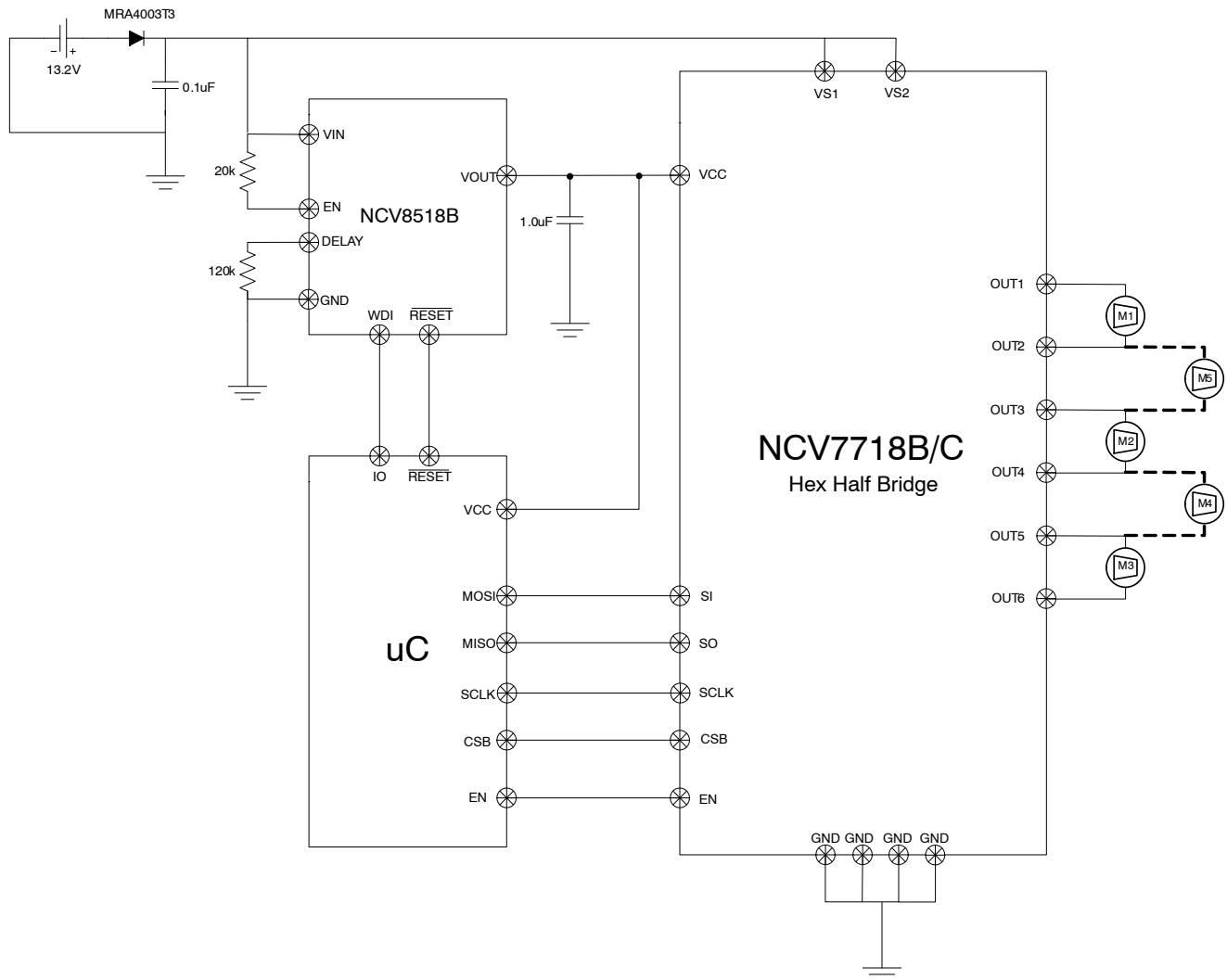
Figure 31. Application Drawing
