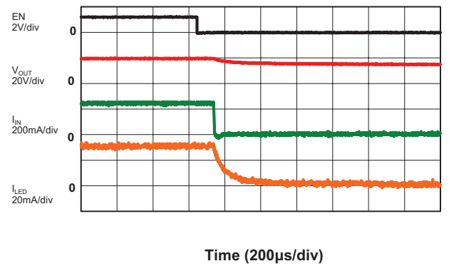
Turn Off ( V_{IN} = 3.6V , C_{IN} = 2.2\mu F , C_{OUT} = 2.2\mu F , R_{FB} = 8.3\Omega , 6 LEDs)
