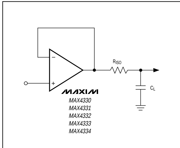
Figure 6. Capacitive-Load-Driving Circuit
