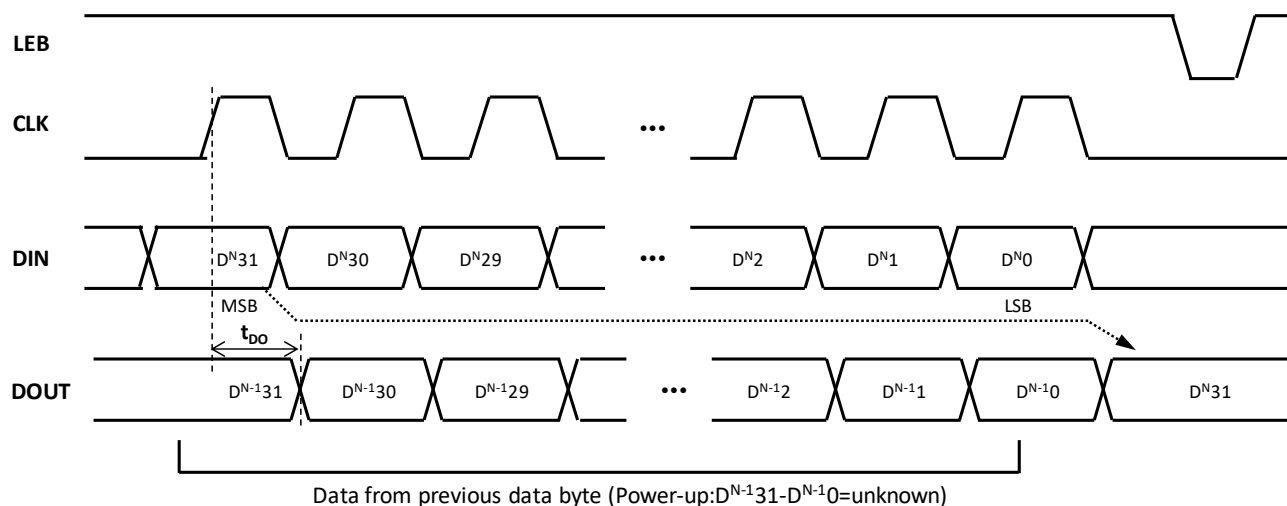
Figure 4 Latch Enable Interface Timing
