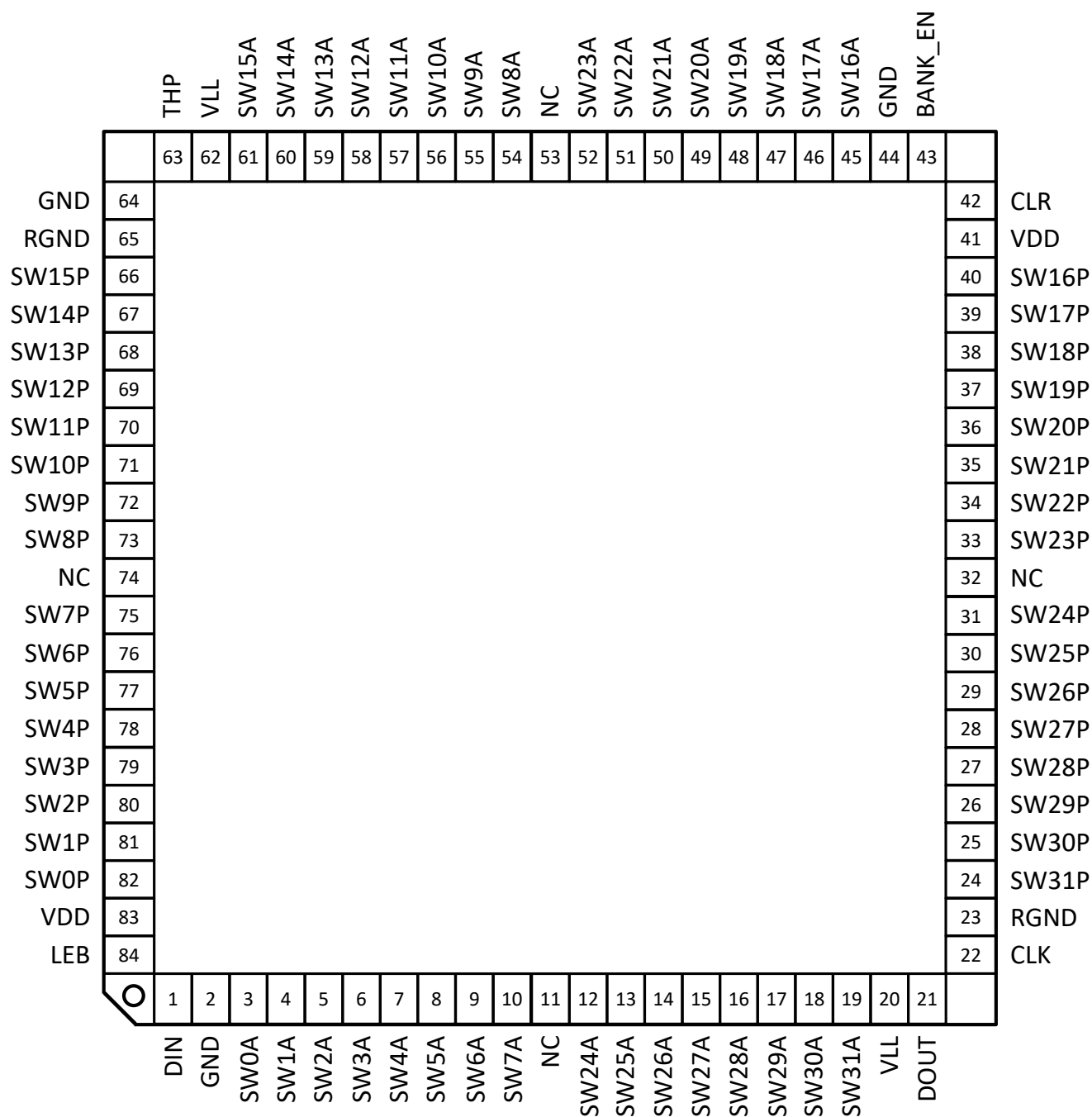
Figure 5 Pin Configuration
