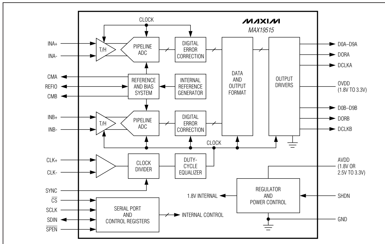
Figure 2. Functional Diagram
