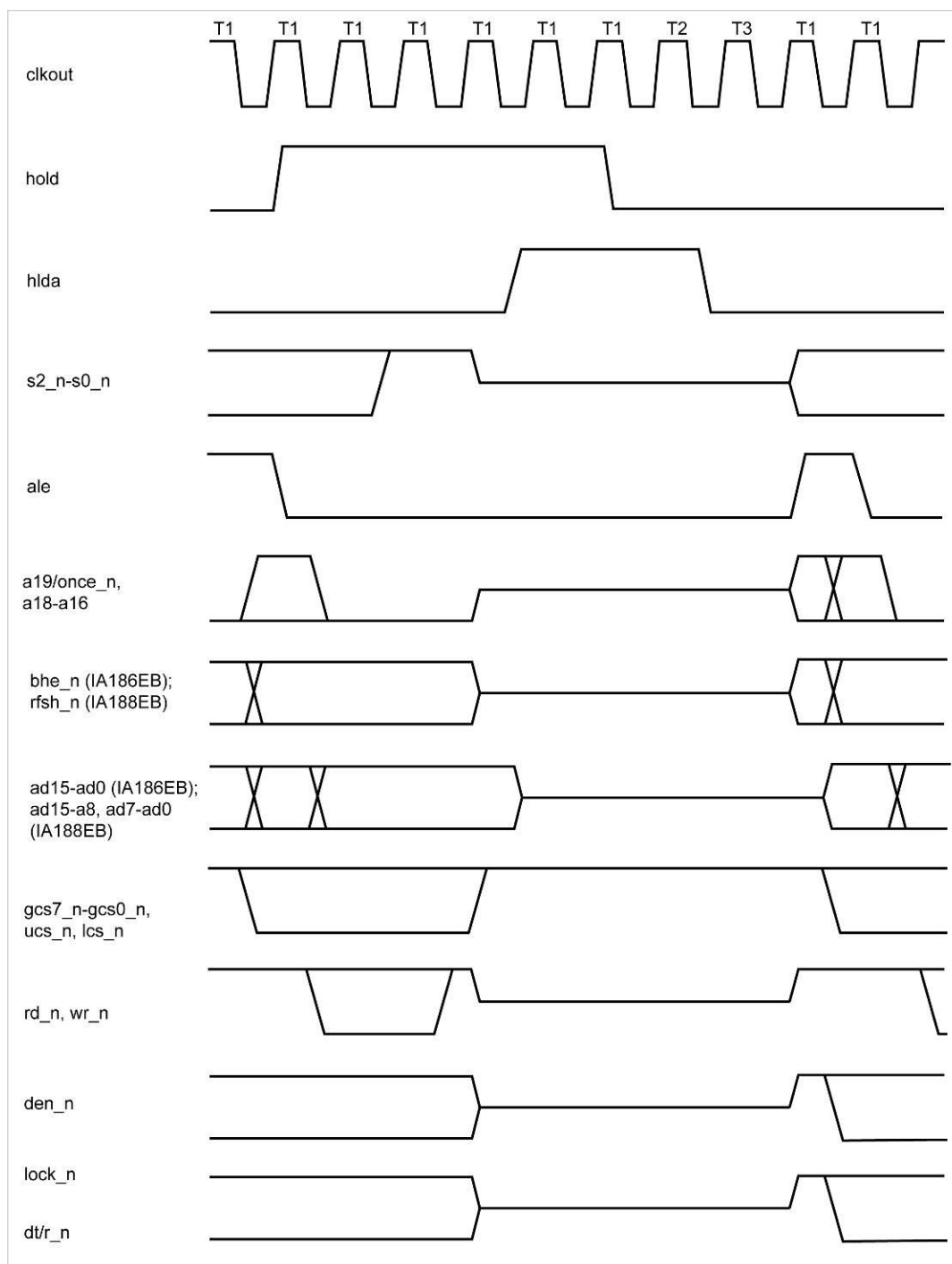
Figure 26. hold/hlida Timing
