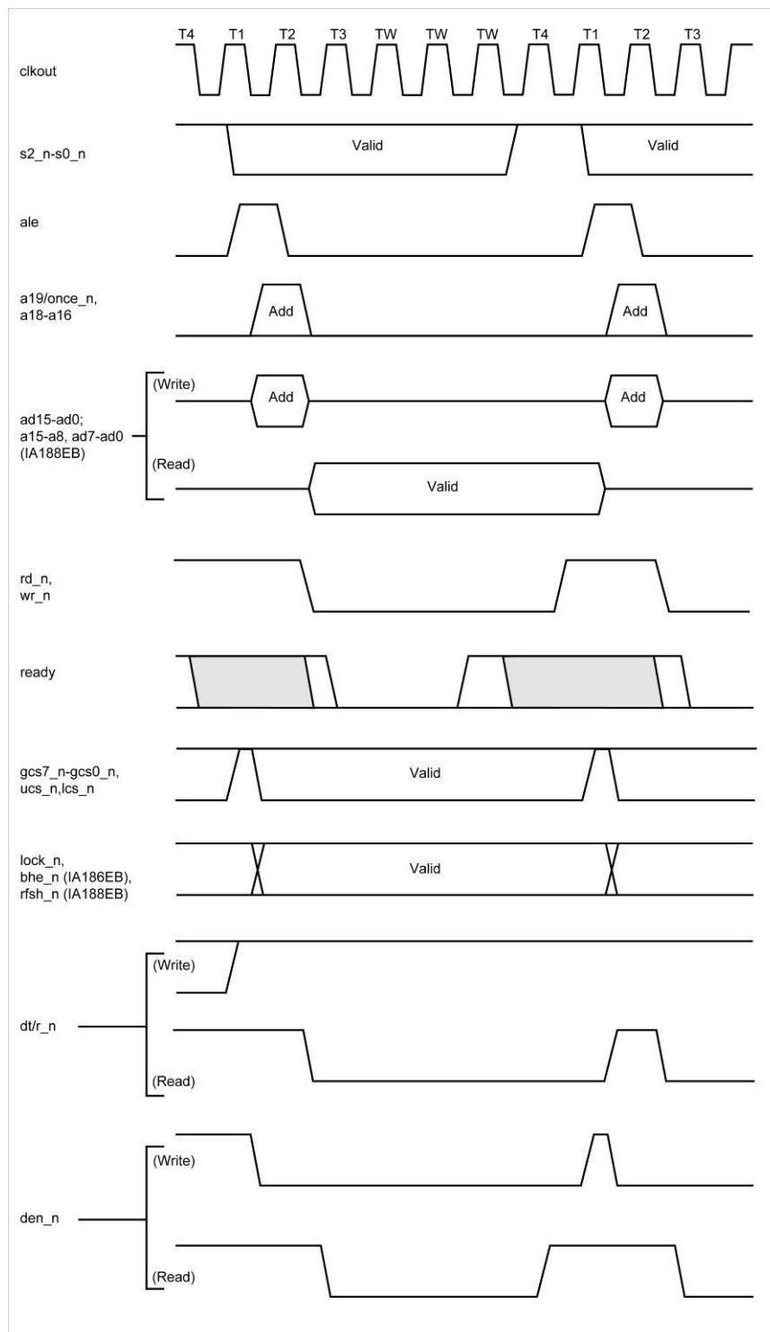
Figure 28. Ready Timing
