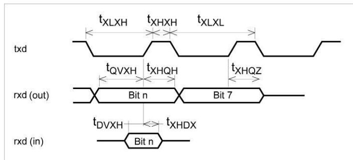
Figure 19. Serial Port Mode 0 Timing Characteristics
