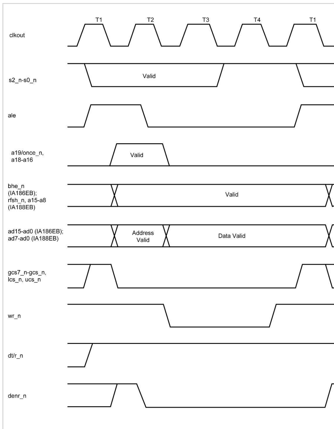
Figure 23. Write Cycle Timing
