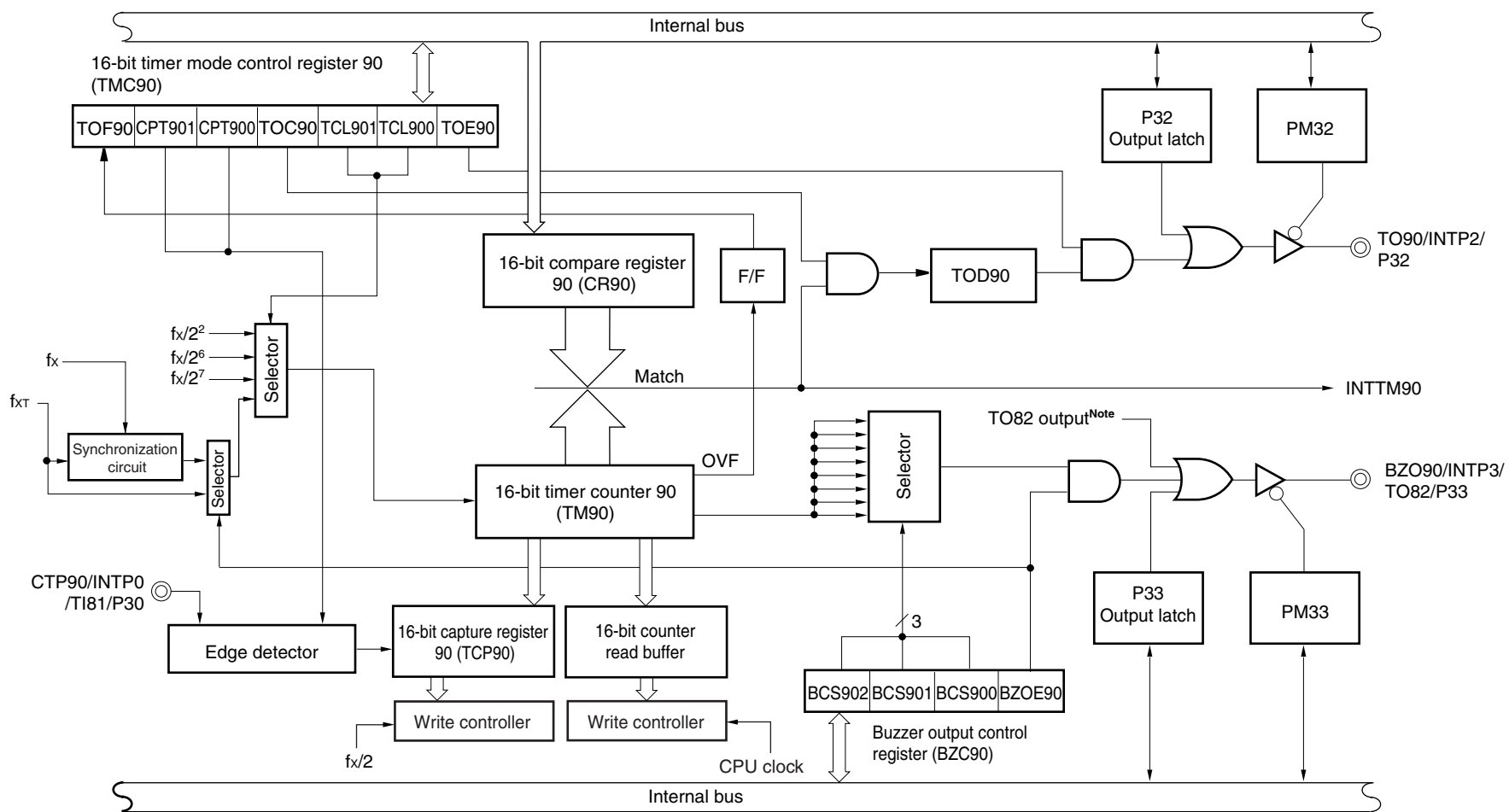
Figure 8-1. Block Diagram of 16-Bit Timer 90
