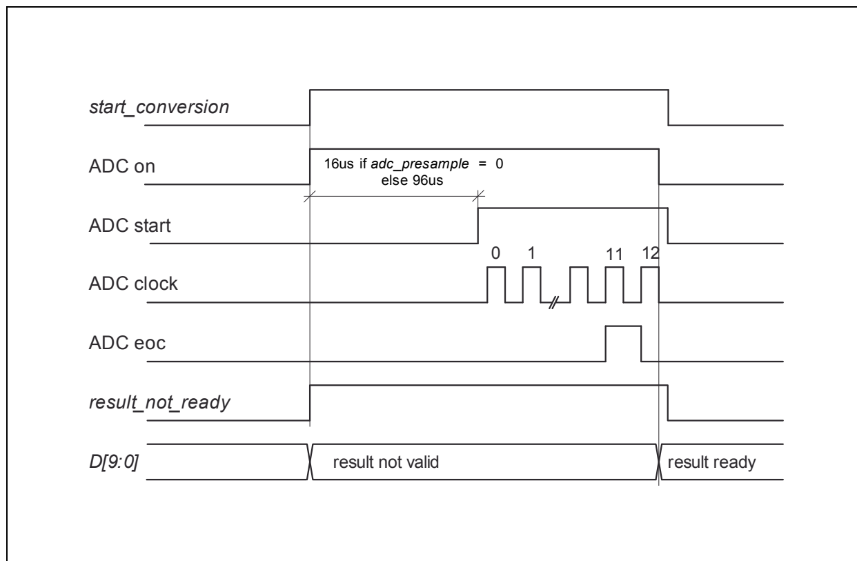
Figure 75: ADC Timing Diagram
