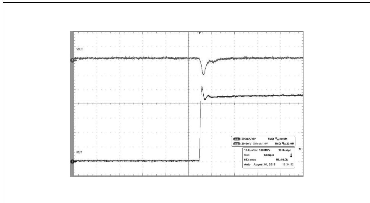
Figure 23: DC/DC Buck SD4 Low Noise Load Transient Fast Mode
