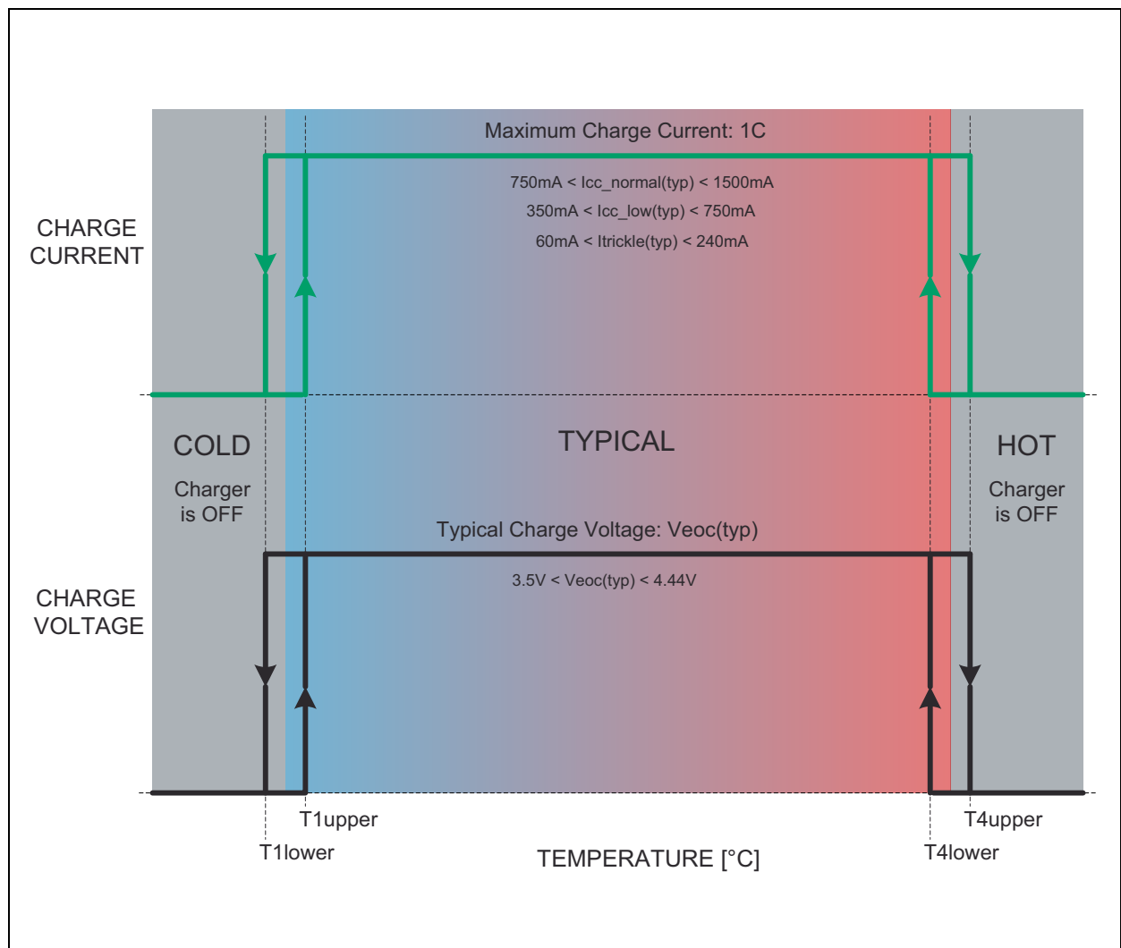
Figure 47: MIN/MAX Temp Supervision
