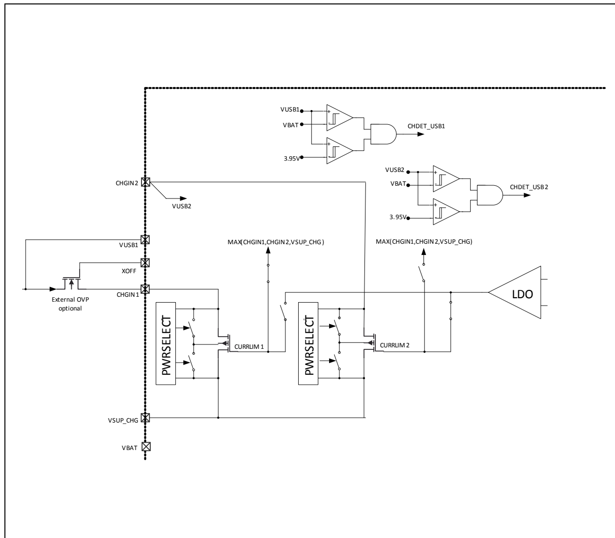
Figure 50: Dual Power Path Diagram
