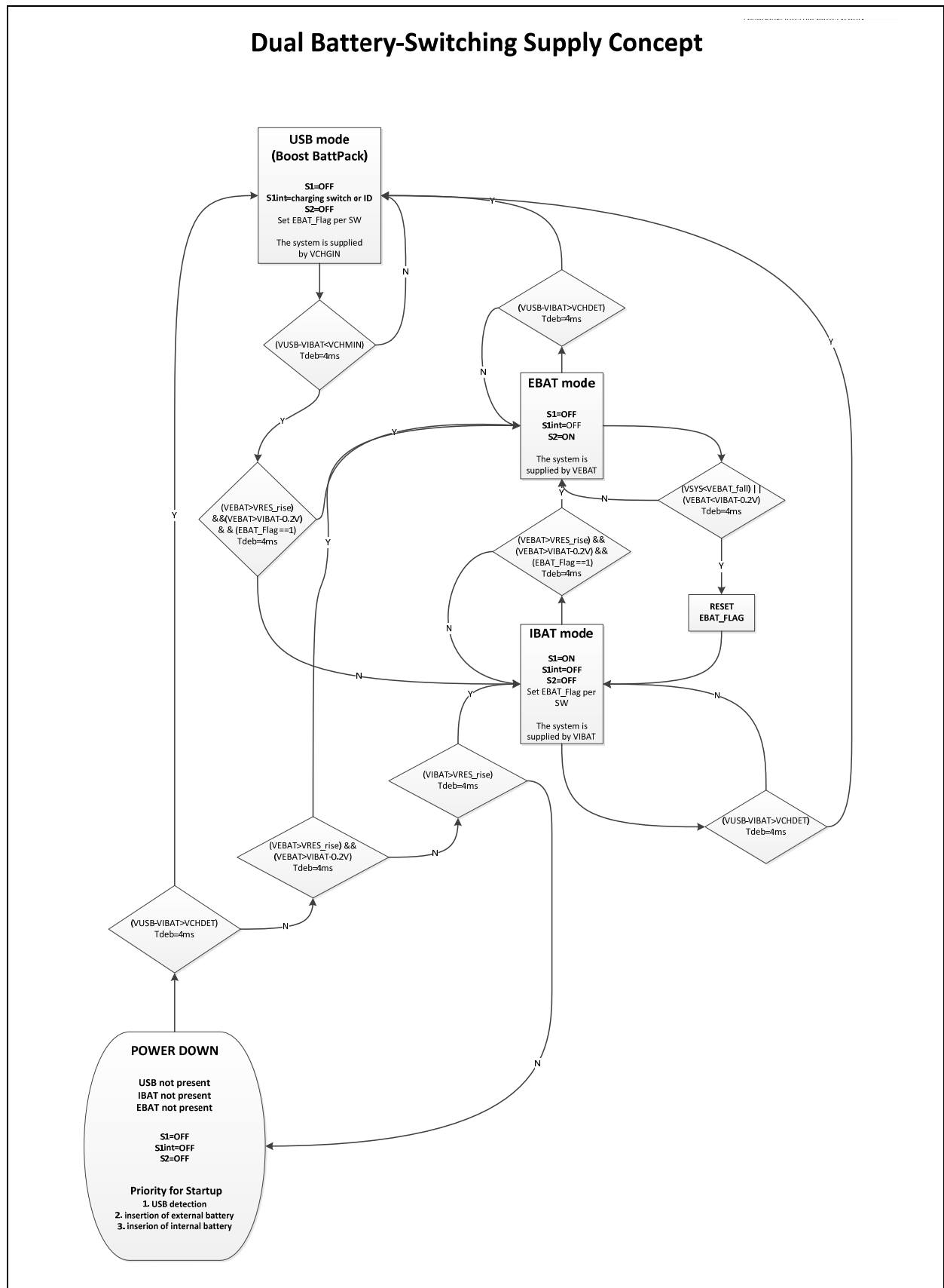
Figure 49: Dual Battery Switching(Flowchart)
