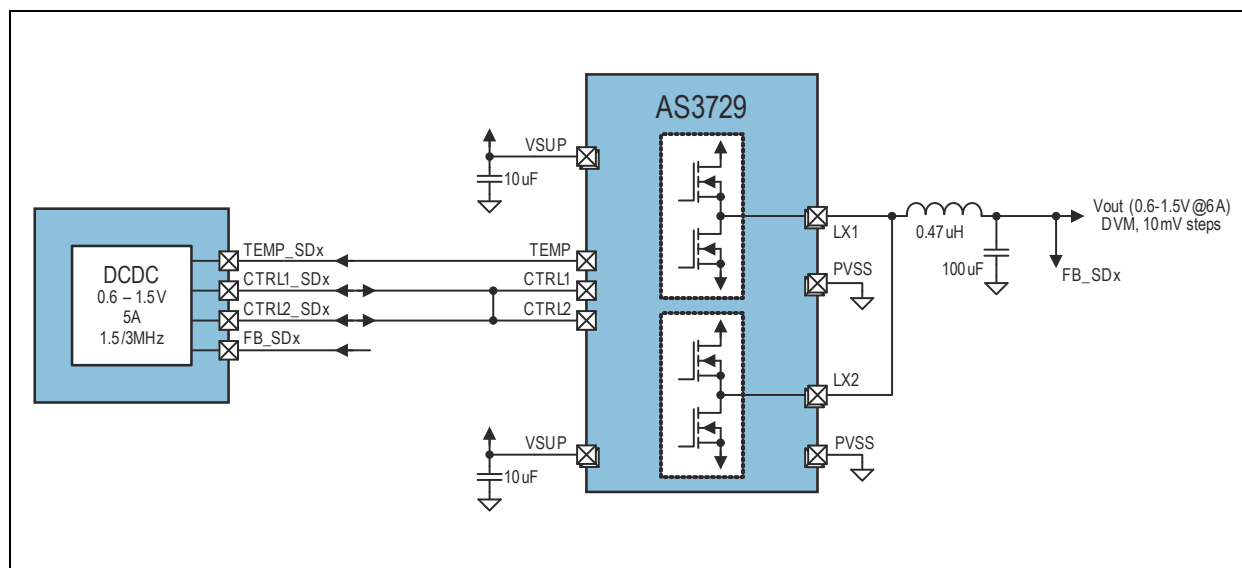
Figure 18: SD4 DC/DC Buck Controller 5A Combined Mode
