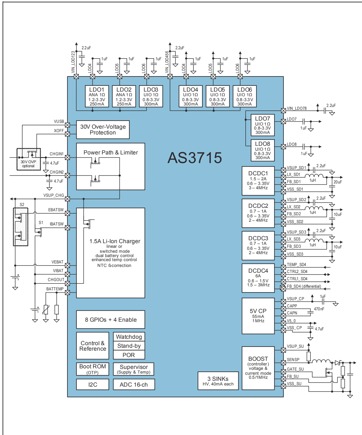
Figure 2: Block Diagram for AS3715
