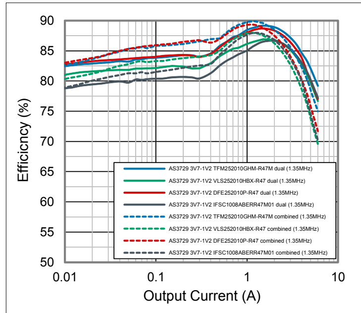
Figure 21: SD4 3.7V Eff vs. Iout Coil Comparison
