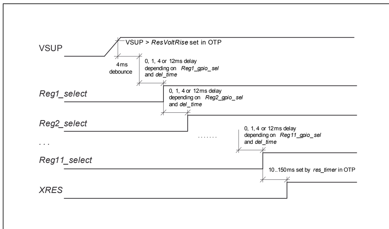
Figure 56: Regulator Power-up Sequence
