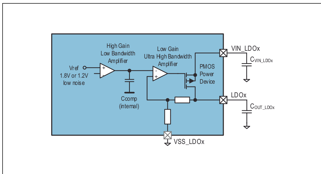
Figure 26: Analog IO LDO Block Diagram
