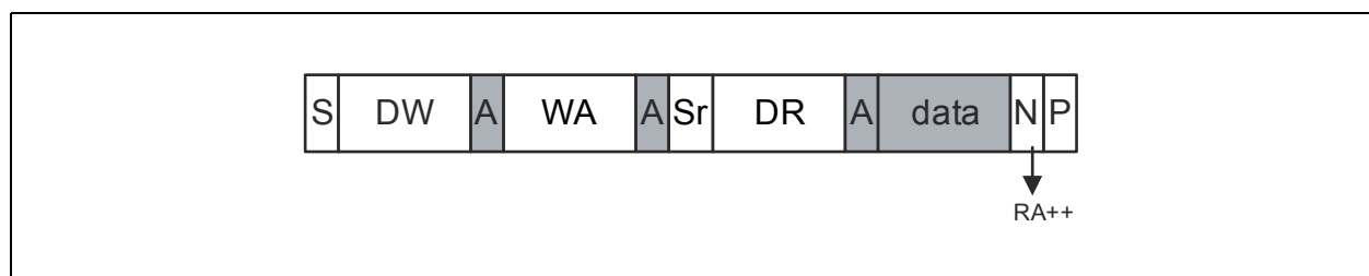
Figure 79: I 2 C Random Read
