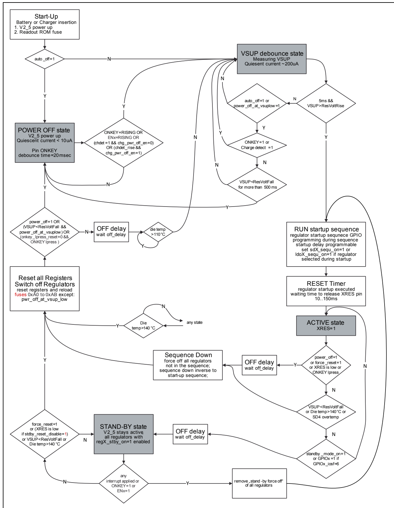
Figure 55: Start-up flow chart
