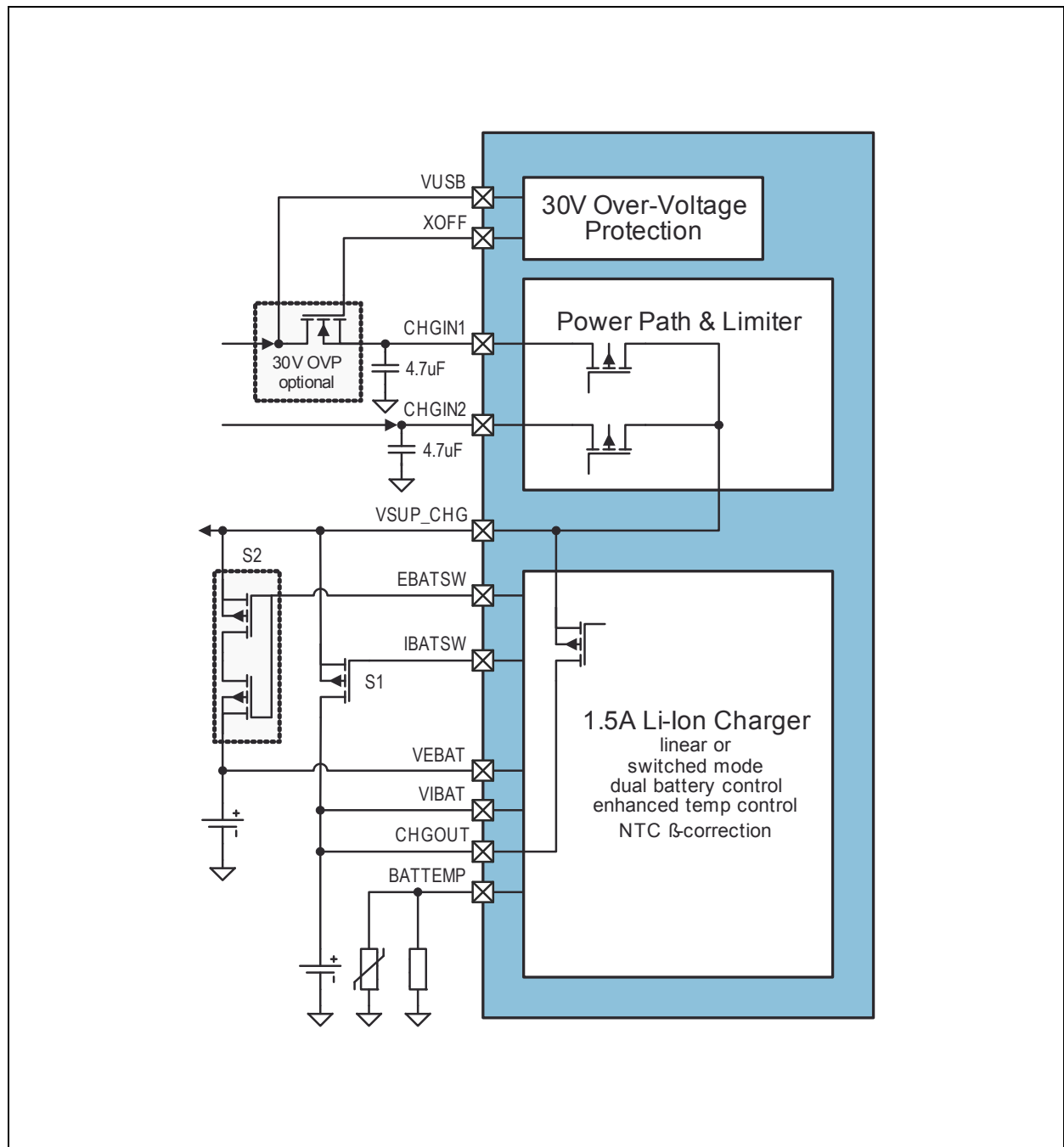
Figure 42: Charger Application Block Diagram, Linear Mode Charger
