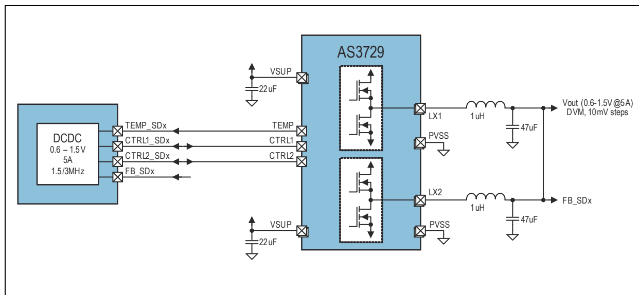
Figure 17: SD4 DC/DC Buck Controller 5A Block Diagram
