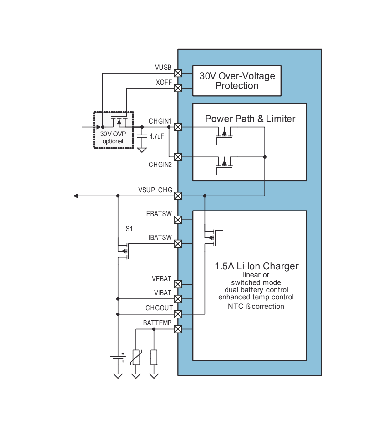
Figure 43: Charger Application Block Diagram, Linear Mode Single Power-path and Battery
