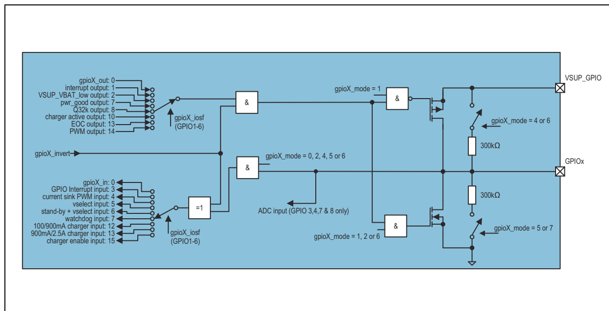
Figure 68: GPIO Block Diagram
