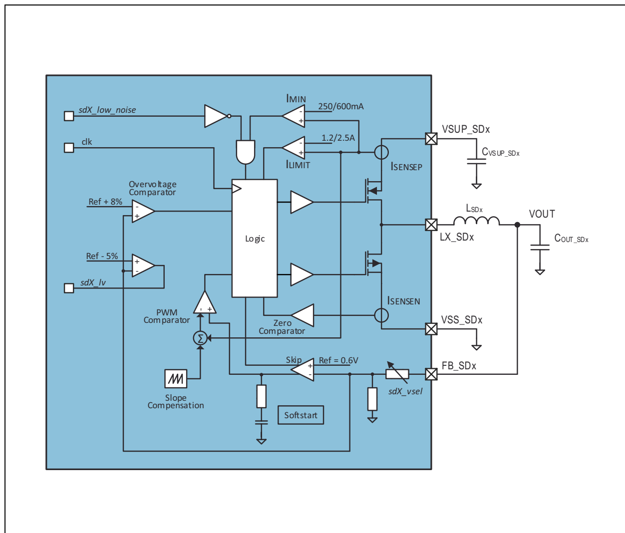
Figure 7: Step Down DC/DC Converter Block Diagram
