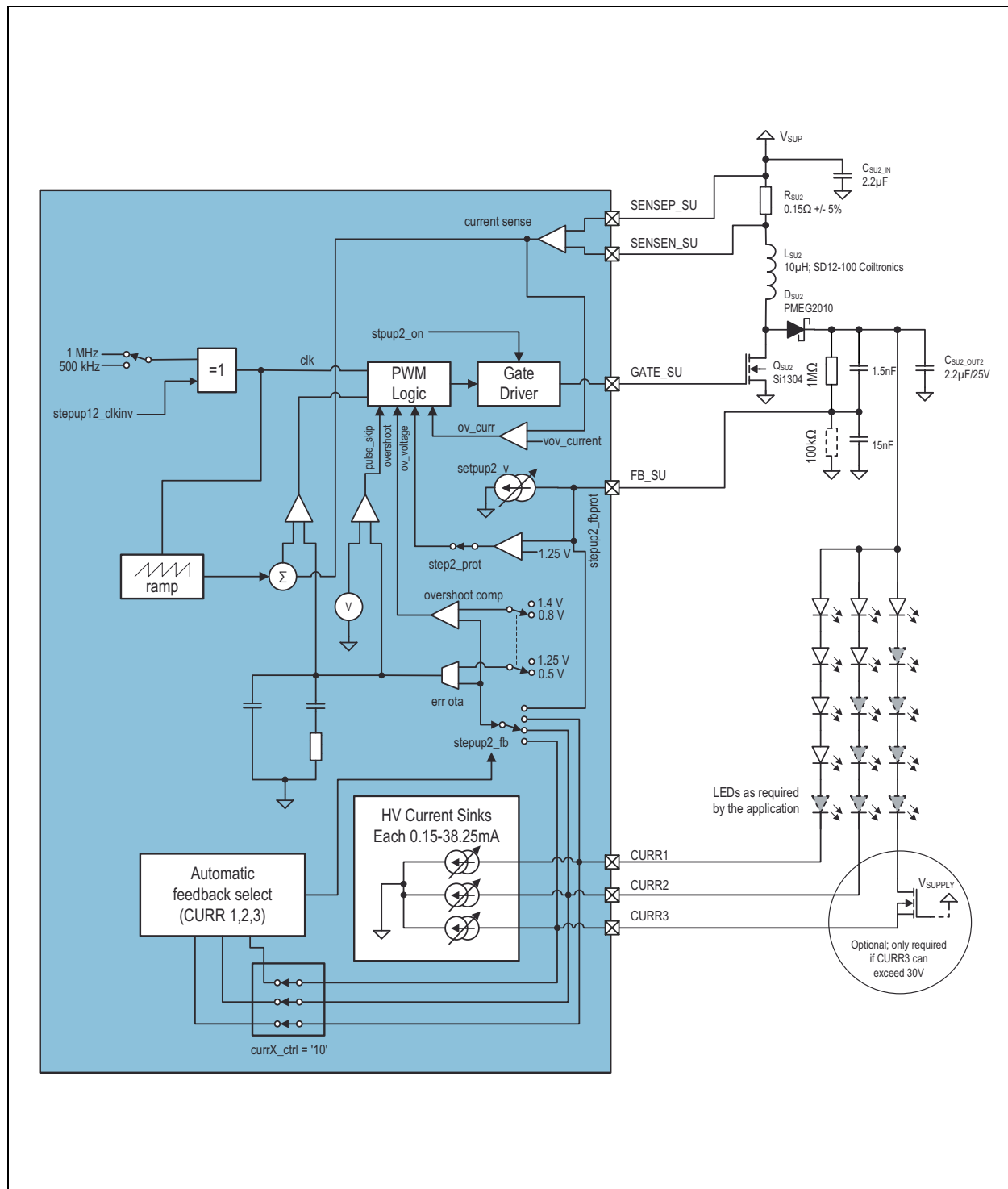
Figure 34: DCDC Step-Up Converter
