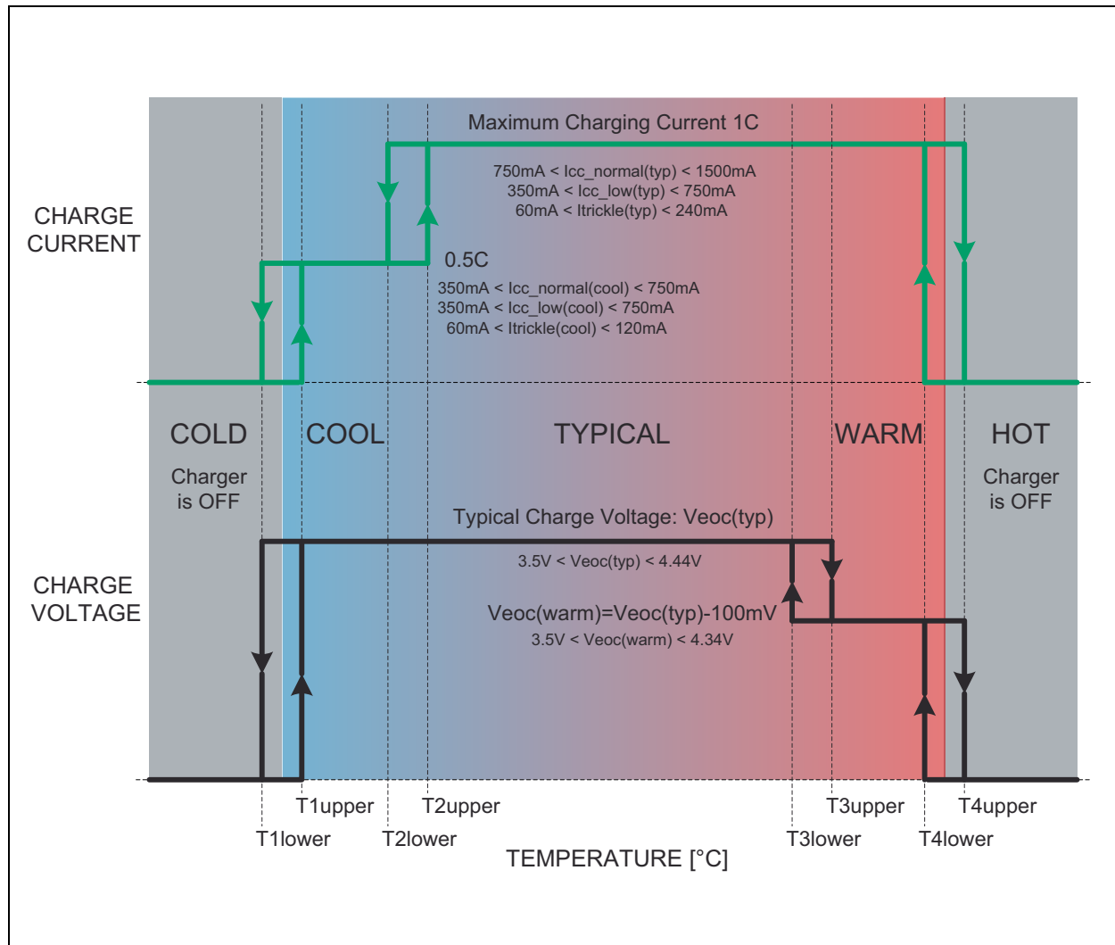
Figure 48: JEITA Temp Supervision
