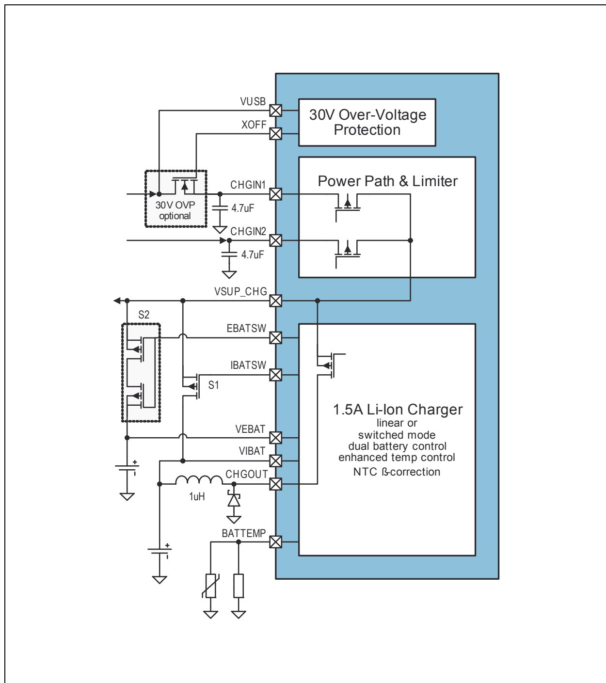
Figure 41: Charger Application Block Diagram, Switch Mode Charger
