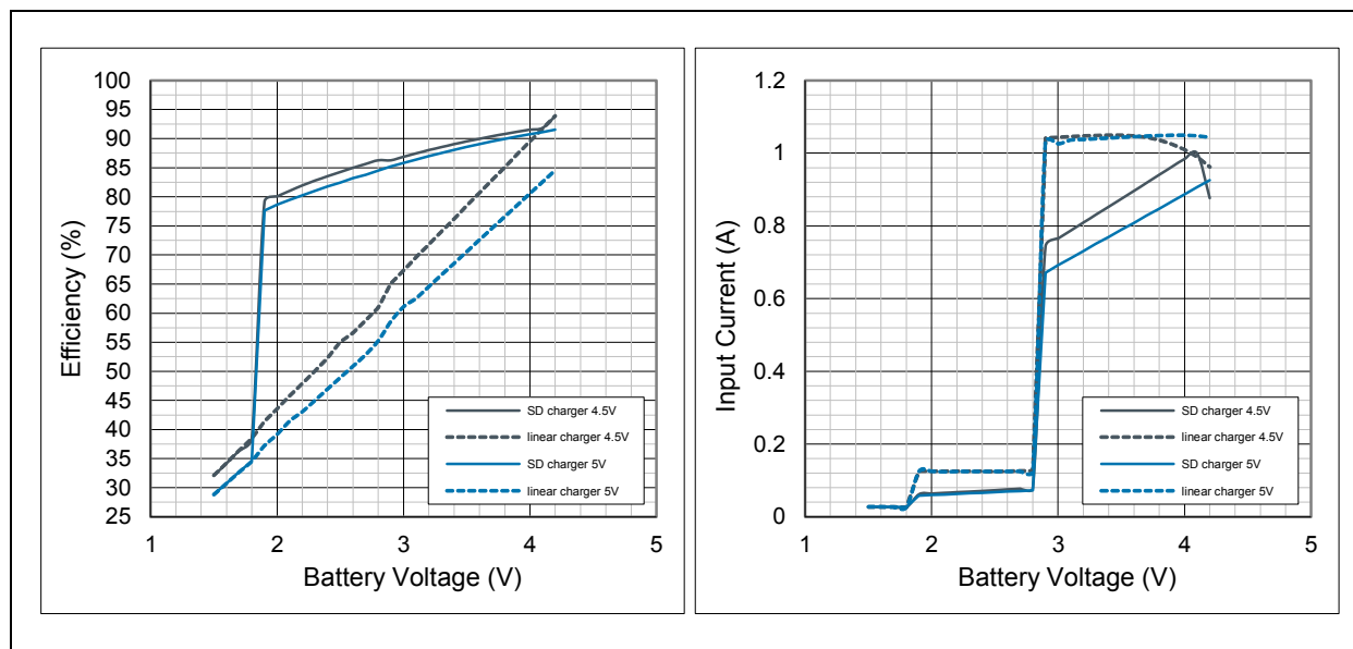
Figure 53: Charger Efficiency and Input Current
