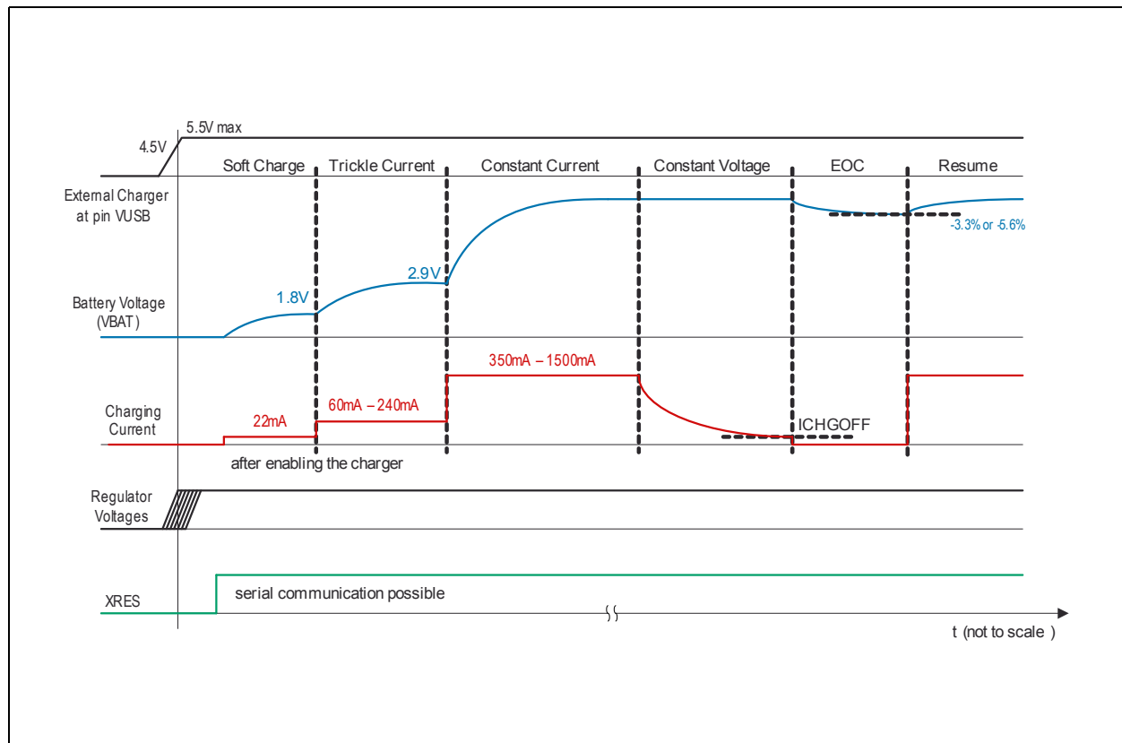
Figure 44: Charger States
