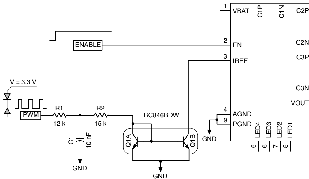
Figure 14. Basic Analog PWM Dimming Control
