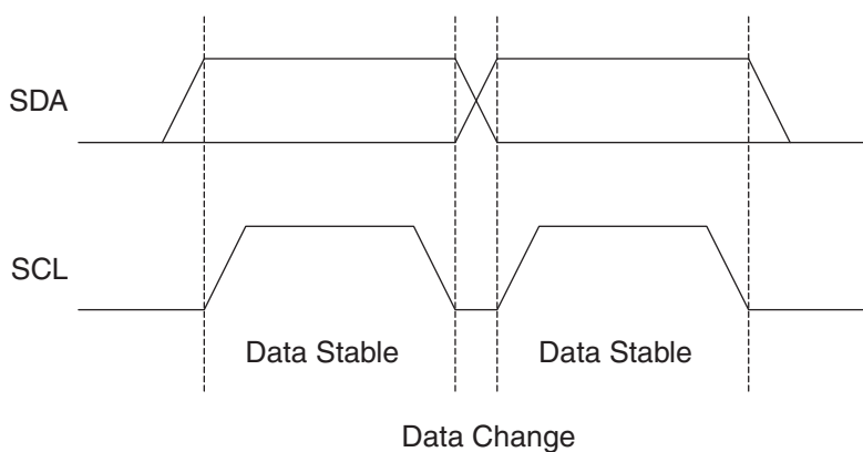
Figure 27-2. Data validity.
