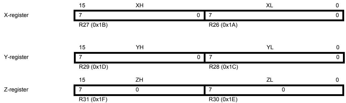
Figure 7-3. The X-register, Y-register, and Z-registers.
