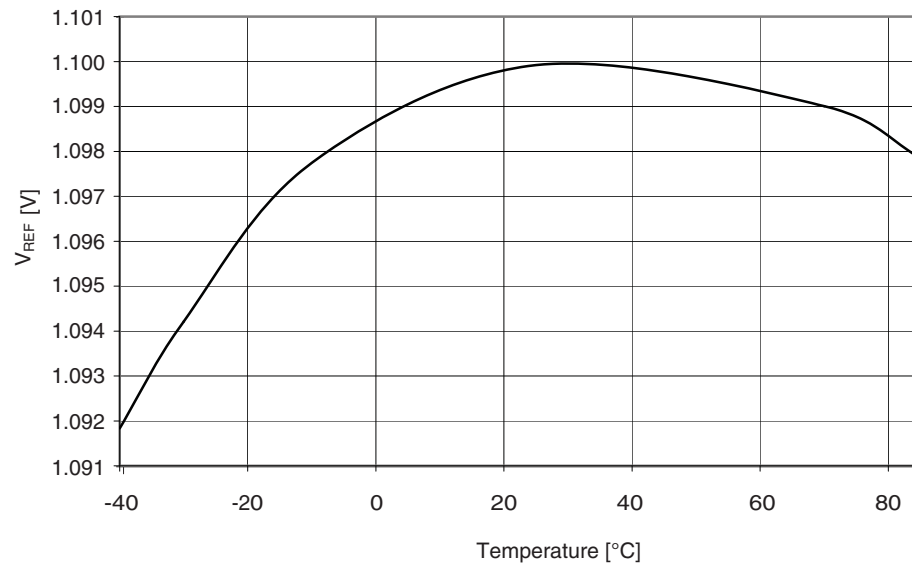
Figure 33-23. Typical VREF deviation curve with Atmel factory calibration at 25°C and 85°C.
