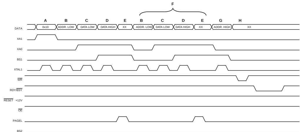
Figure 30-5. Programming the flash waveforms (1) .
