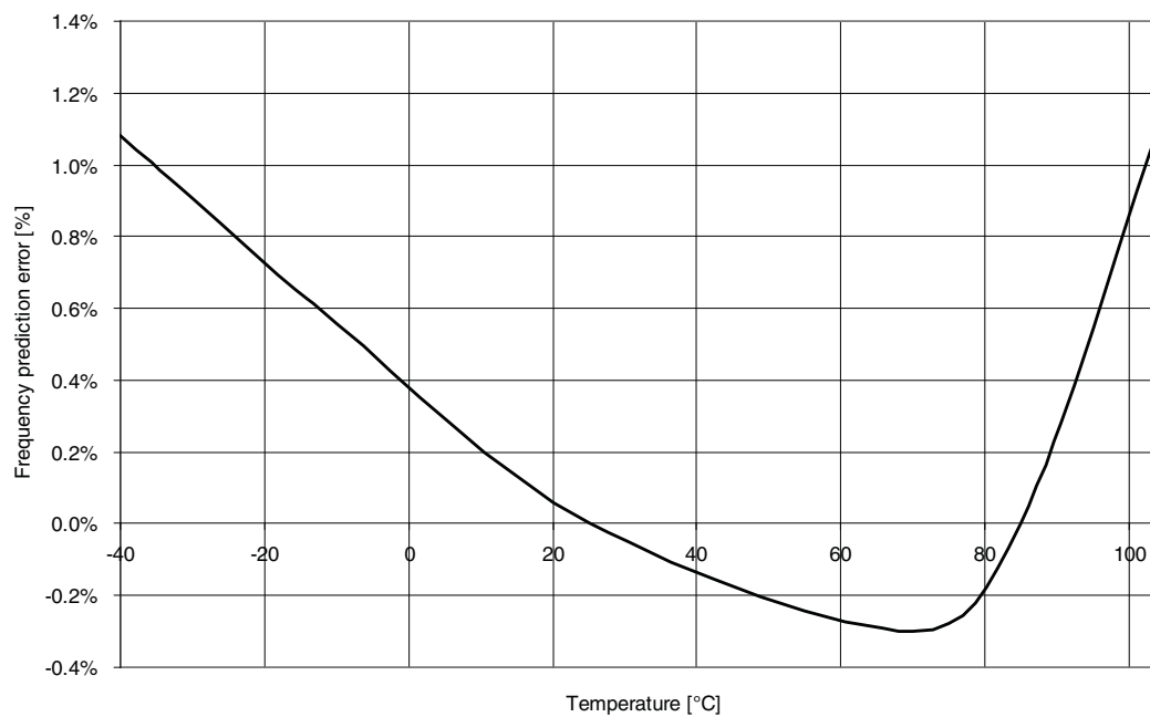
Figure 33-21. Typical SlowRC frequency frequency prediction error based on algorithm in Section 9.2.2 on page 27 .
