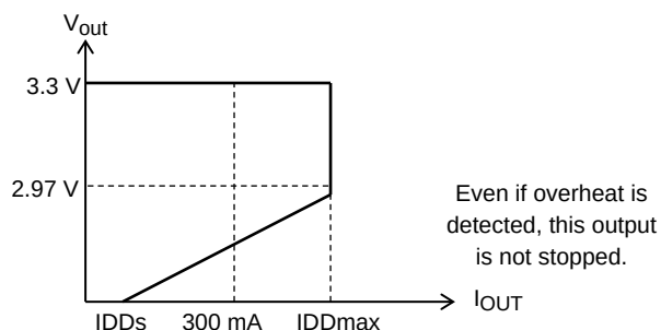
VDD output voltage - Load characteristics
