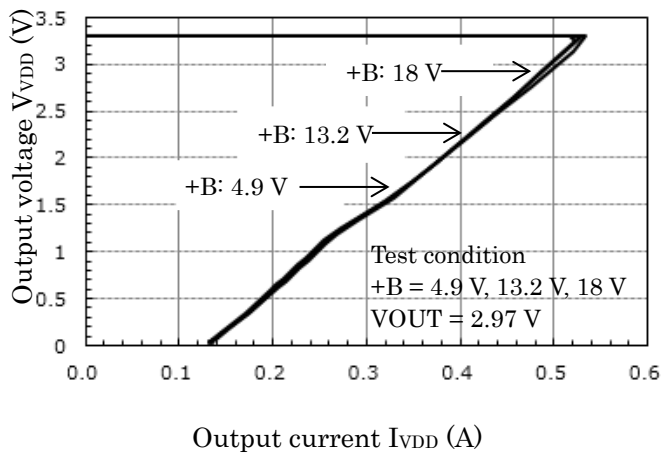
V_{VDD} - I_{VDD}
