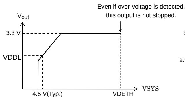
VDD I/O characteristics
