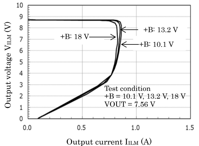
V_{ILM} - I_{ILM} (8.5 V setting)
