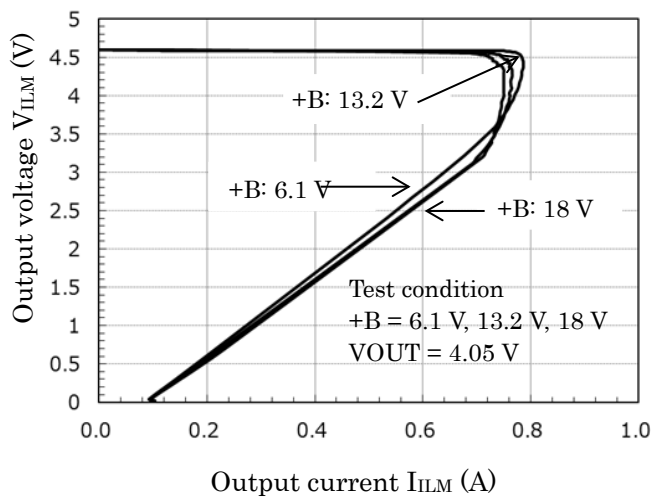
V_{ILM} - I_{ILM} (4.5 V setting)
