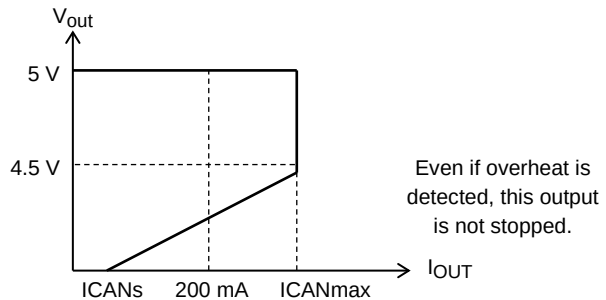
CAN output voltage - Load characteristics
