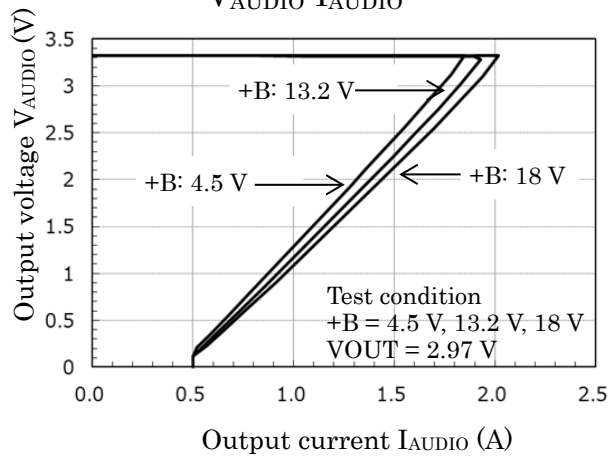
V_{AUDIO}-I_{AUDIO}
