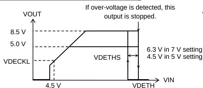
I/O characteristics in DECK 8.5 V setting
