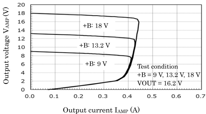
V_{AMP}-I_{AMP}
