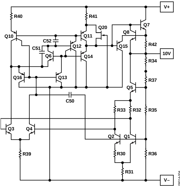
Figure 4. Simplified Schematic
