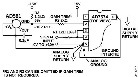
Figure 15. AD581 as -10 V Reference for CMOS ADC
