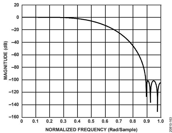
Figure 73. Third 2x Half-Band 22.5% Filter Response
