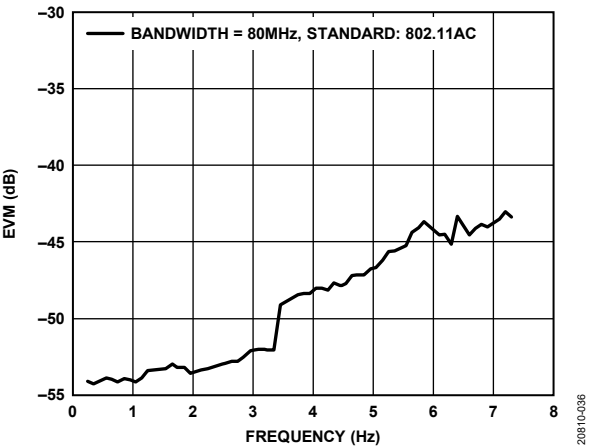
Figure 42. EVM vs. Frequency, 80 MHz Channel, Swept Across First, Second, and Third Nyquist, f_{DAC} = 11796.48\text{ MSPS}
