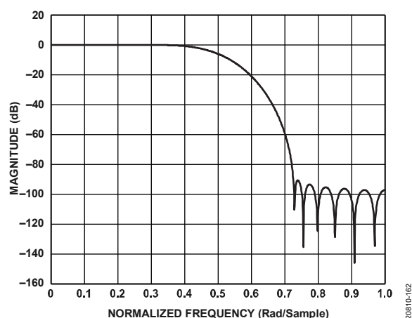
Figure 72. Second 2x Half-Band 45% Filter Response
