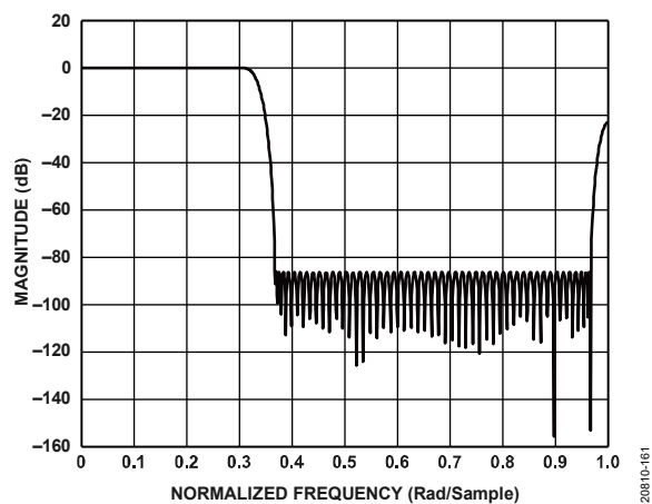
Figure 71. 3x Third-Band 90% Filter Response
