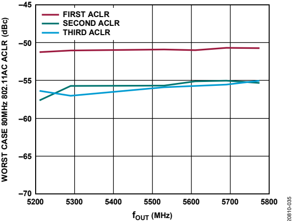
Figure 41. Worst Case 80 MHz 802.11AC ACLR vs. f_{OUT}
