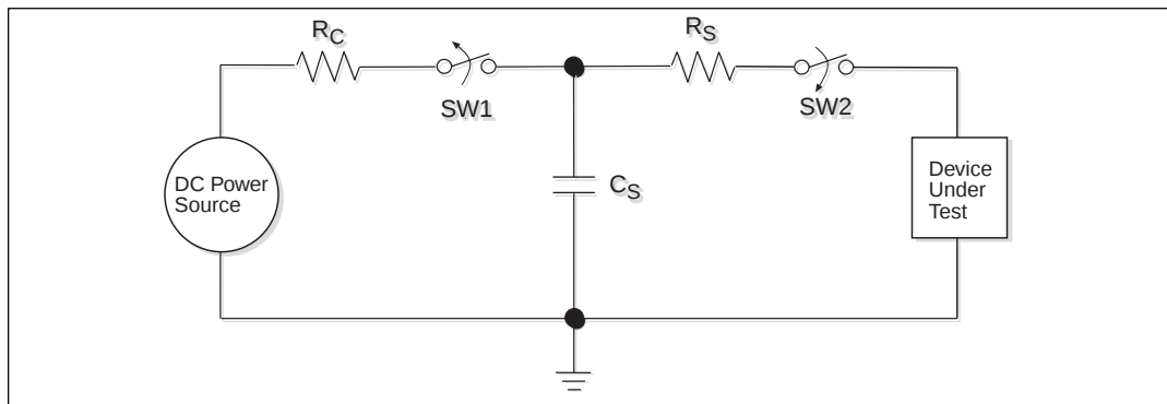
Figure 16. ESD Test Circuit for Human Body Model
