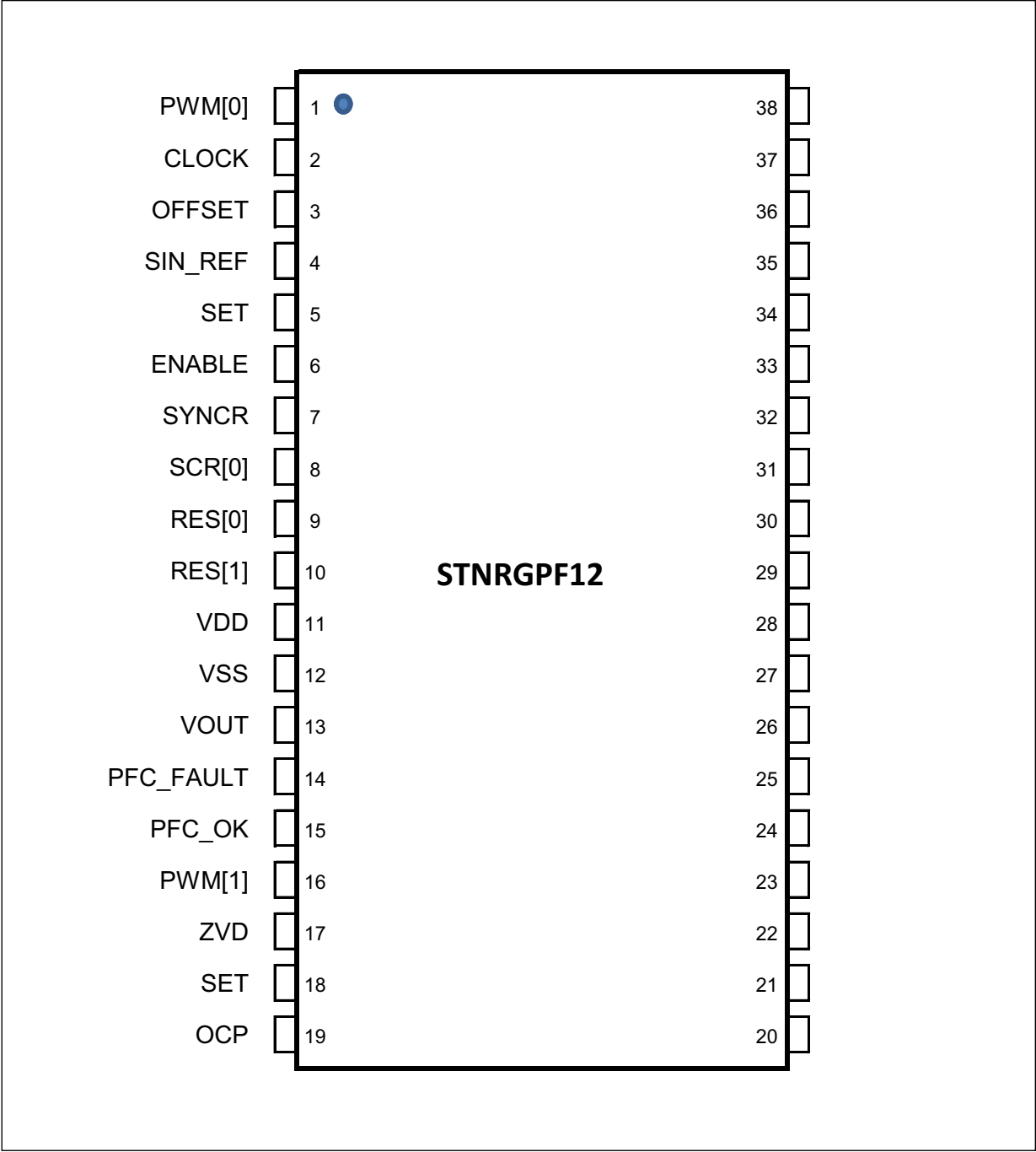
Figure 1. STNRGPF12 pinout
