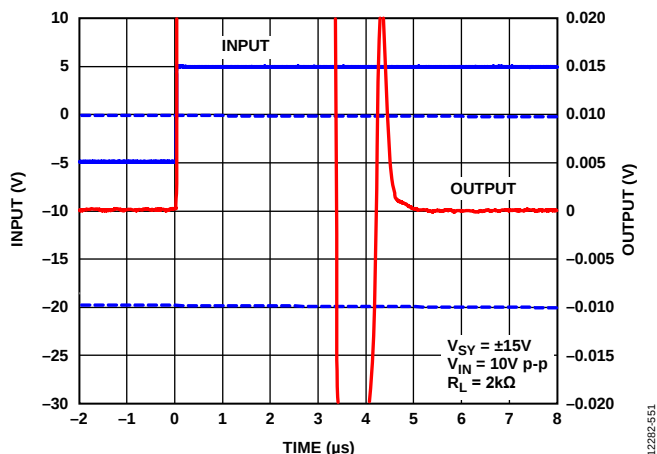
Figure 62. Positive Settling Time to 0.1%, V_{SV} = \pm 15V
