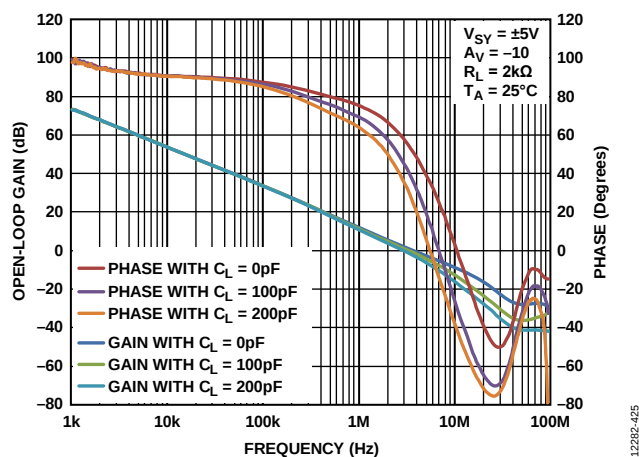
Figure 39. Open-Loop Gain and Phase vs. Frequency, V_{SV} = \pm 5 V
