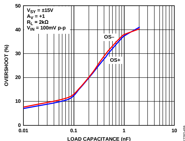
Figure 61. Small Signal Overshoot vs. Load Capacitance, V_{SV} = \pm 15V
