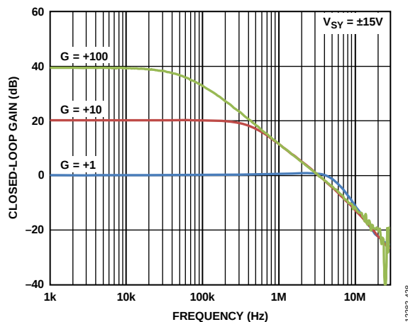
Figure 43. Closed-Loop Gain vs. Frequency, V_{SV} = \pm 15 V
