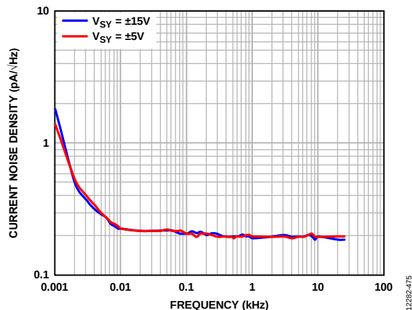
Figure 76. Current Noise Density vs. Frequency, V_{SY} = \pm 5\text{ V} and V_{SY} = \pm 15\text{ V}
