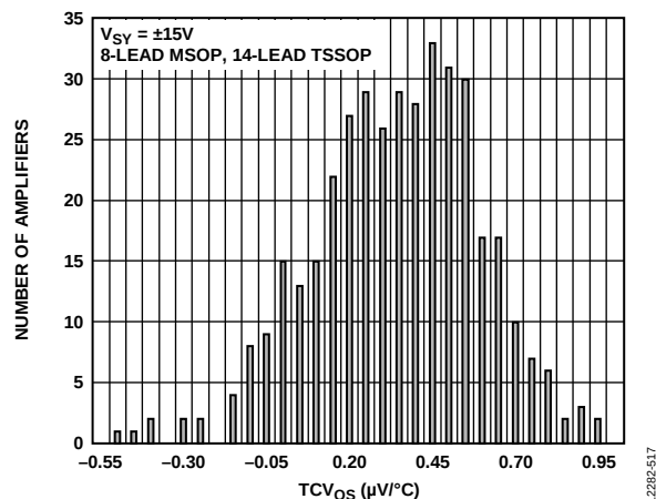
Figure 25. Temperature Coefficient of Offset Voltage ( TCV_{OS} ), V_{SY} = \pm 15V , 8-Lead MSOP and 14-Lead TSSOP
