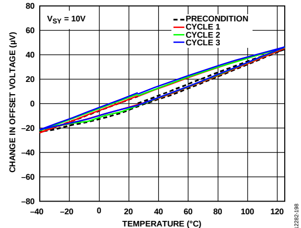
Figure 98. Change in Offset Voltage over Three Full Temperature Cycles
