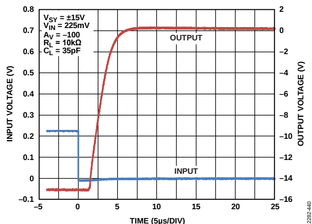
Figure 55. Negative Overload Recovery, V_{SV} = \pm 15\text{ V}
