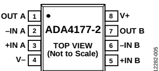
Figure 6. ADA4177-2 8-Lead SOIC Pin Configuration
