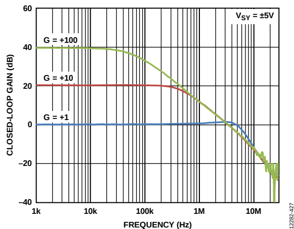
Figure 40. Closed-Loop Gain vs. Frequency, V_{SV} = \pm 5 V
