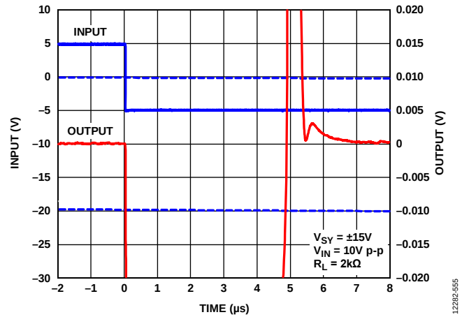
Figure 66. Negative Settling Time 0.1%, V_{SY} = \pm 15\text{ V}
