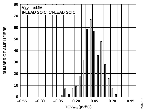
Figure 24. Temperature Coefficient of Offset Voltage ( TCV_{OS} ), V_{SY} = \pm 15V , 8-Lead SOIC and 14-Lead SOIC
