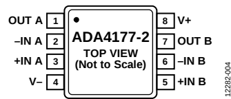
Figure 5. ADA4177-2 8-Lead MSOP Pin Configuration
