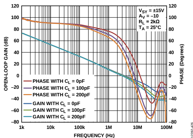
Figure 42. Open-Loop Gain and Phase vs. Frequency, V_{SV} = \pm 15 V
