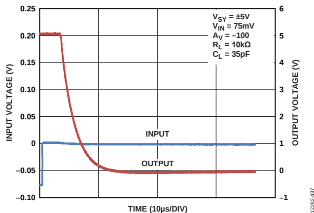
Figure 51. Positive Overload Recovery, V_{SV} = \pm 5\text{ V}
