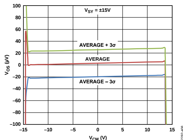
Figure 26. Input Offset Voltage ( V_{OS} ) vs. Common-Mode Voltage ( V_{CM} ), V_{SY} = \pm 15V
