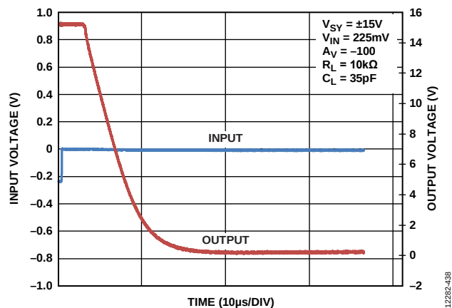
Figure 54. Positive Overload Recovery, V_{SV} = \pm 15\text{ V}
