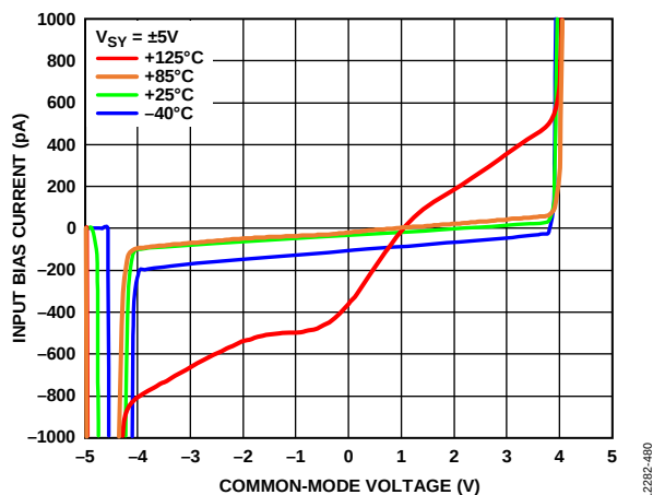
Figure 75. Input Bias Current vs. Common-Mode Voltage ( V_{CM} ) and Temperature, V_{SY} = \pm 5\text{ V}
