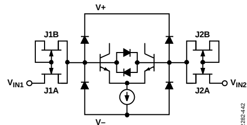
Figure 87. Conceptual Schematic of the Inputs of the ADA4177-1/ADA4177-2/ADA4177-4
