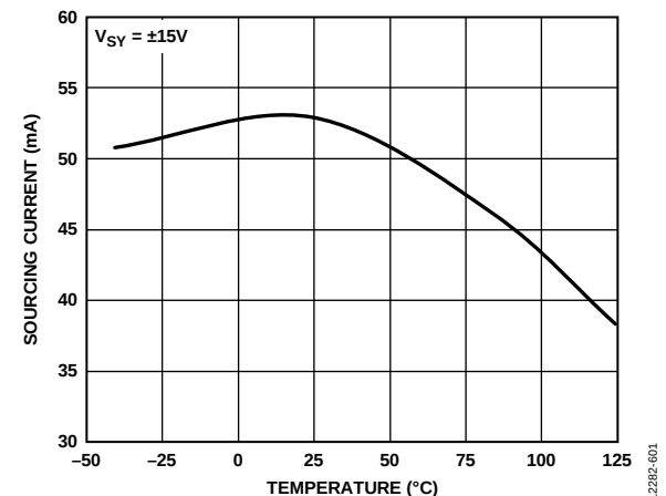
Figure 80. Output Short-Circuit Sourcing Current vs. Temperature, V_{SY} = \pm 15\text{ V}
