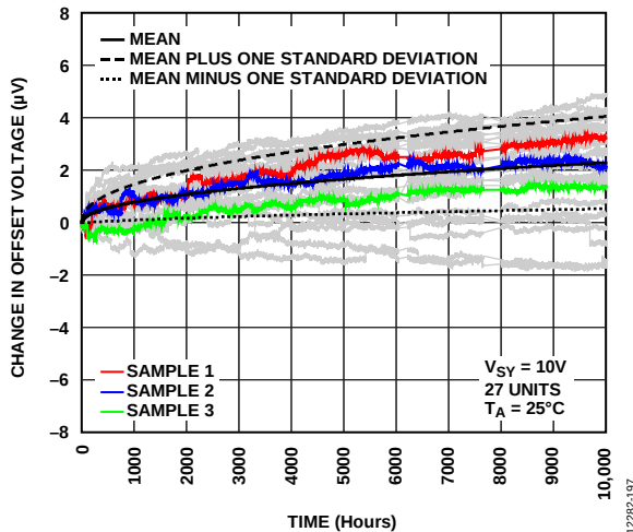
Figure 97. Measured Long-Term Drift of the ADA4177-1/ADA4177-2/ADA4177-4 Offset Voltage over 10,000 Hours
