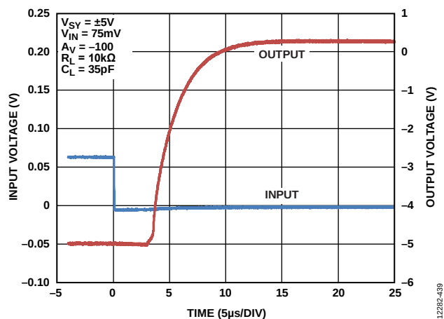
Figure 52. Negative Overload Recovery, V_{SV} = \pm 5\text{ V}
