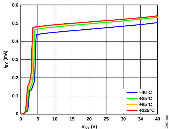
Figure 33. Supply Current per Amplifier ( I_S ) vs. Power Supply Voltage ( V_{SY} )
