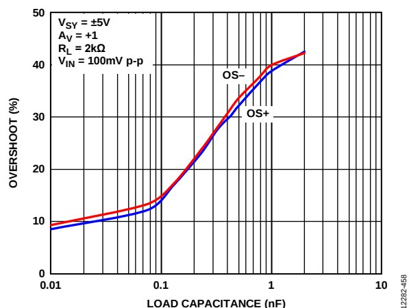
Figure 58. Small Signal Overshoot vs. Load Capacitance, V_{SV} = \pm 5V
