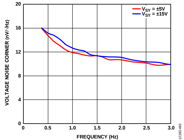
Figure 67. Voltage Noise Corner vs. Frequency, V_{SY} = \pm 5\text{ V} and V_{SY} = \pm 15\text{ V}
