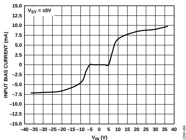
Figure 71. Input Bias Current vs. Input Voltage ( V_{IN} ) Including Input Overvoltage Range (Beyond V_{SY} = \pm 5\text{ V} )
