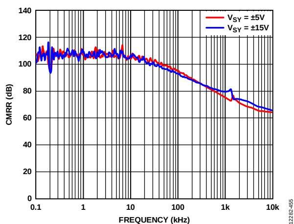
Figure 56. Common-Mode Rejection Ratio (CMRR) vs. Frequency, V_{SV} = \pm 5\text{ V and } V_{SV} = \pm 15\text{ V}
