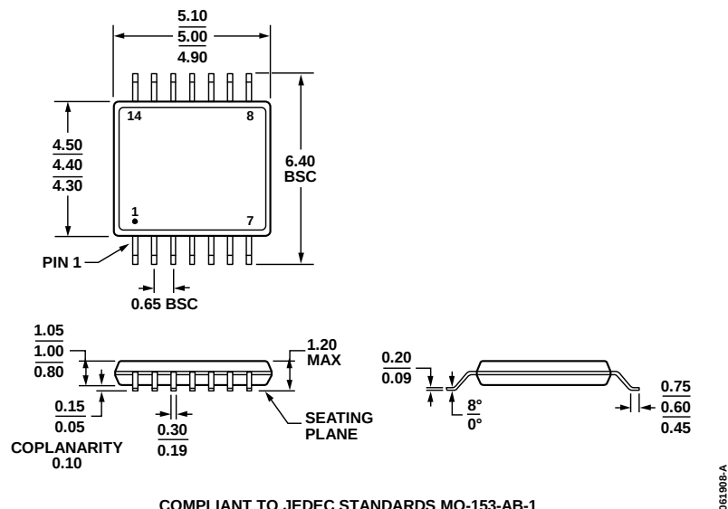
Figure 102. 14-Lead Thin Shrink Small Outline Package [TSSOP] (RU-14)
