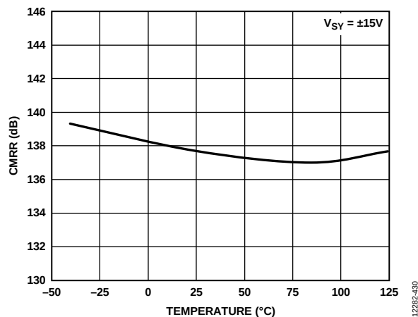
Figure 44. Common-Mode Rejection Ratio (CMRR) vs. Temperature, V_{SV} = \pm 15 V
