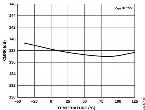
Figure 41. Common-Mode Rejection Ratio (CMRR) vs. Temperature, V_{SV} = \pm 5 V
