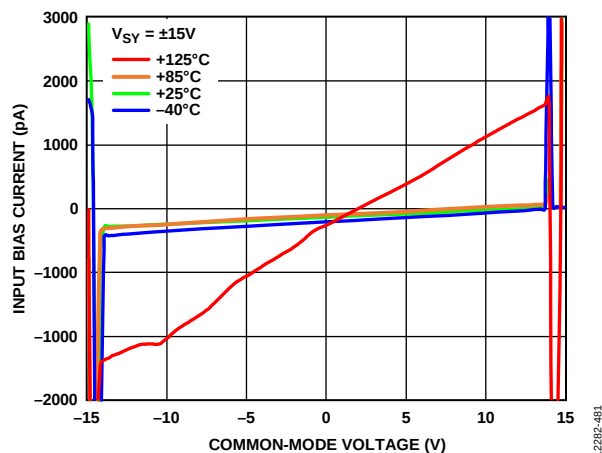
Figure 78. Input Bias Current vs. Common-Mode Voltage ( V_{CM} ) and Temperature, V_{SY} = \pm 15\text{ V}
