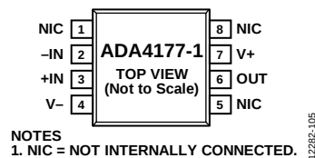
Figure 4. ADA4177-1 8-Lead SOIC Pin Configuration
