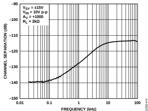
Figure 79. Channel Separation vs. Frequency, V_{SY} = \pm 15\text{ V}
