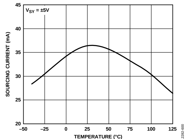
Figure 77. Output Short-Circuit Sourcing Current vs. Temperature, V_{SY} = \pm 5\text{ V}
