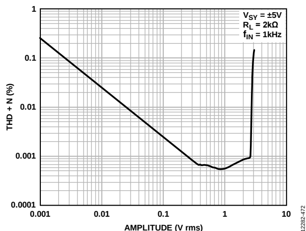
Figure 69. THD + N vs. Amplitude, V_{SY} = \pm 5\text{ V}
