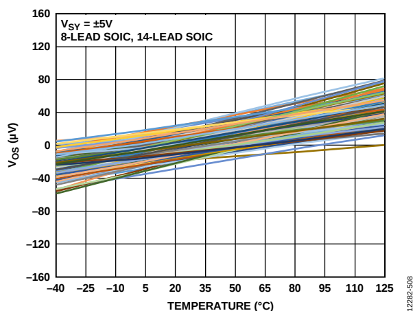
Figure 16. Input Offset Voltage ( V_{OS} ) vs. Temperature, V_{SY} = \pm 5V , 8-Lead SOIC and 14-Lead SOIC
