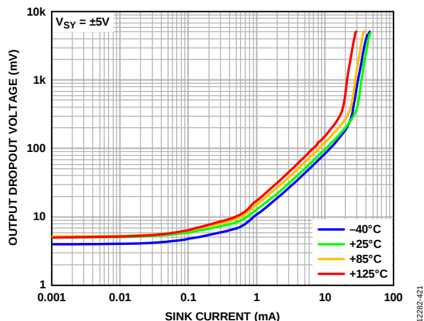
Figure 34. Output Dropout Voltage vs. Sink Current, V_{SY} = \pm 5V
