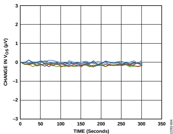
Figure 82. Offset Voltage Short-Term Drift
