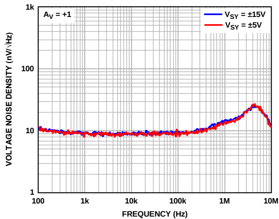
Figure 64. Voltage Noise Density vs. Frequency, V_{SY} = \pm 5\text{ V} and V_{SY} = \pm 15\text{ V}
