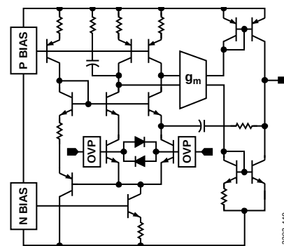
Figure 84. Conceptual Schematic
