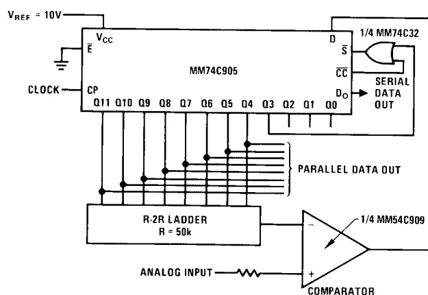
12-Bit Successive Approximation A-to-D Converter, Operating in Continuous Mode, Drives the 50k/100k Ladder Network Directly
