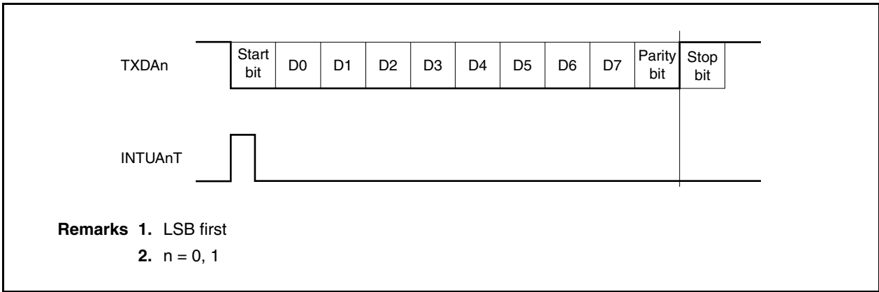
Figure 12-7. UART Transmission
