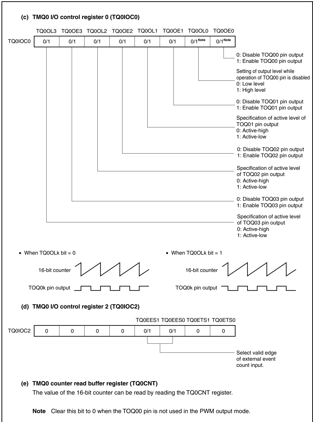
Figure 7-26. Setting of Registers in PWM Output Mode (2/3)
