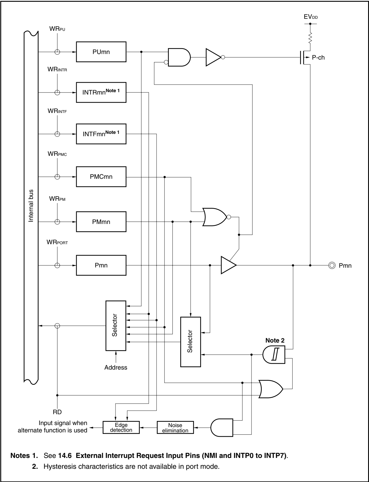
Figure 4-13 Block Diagram of Type I -1
