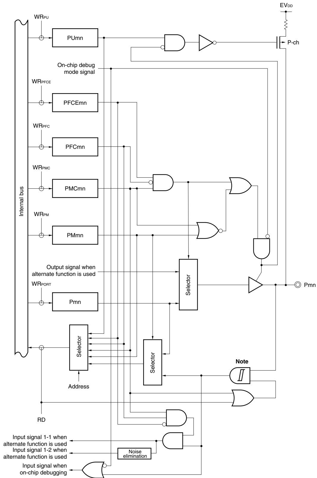
Figure 4-18. Block Diagram of Type U-5
