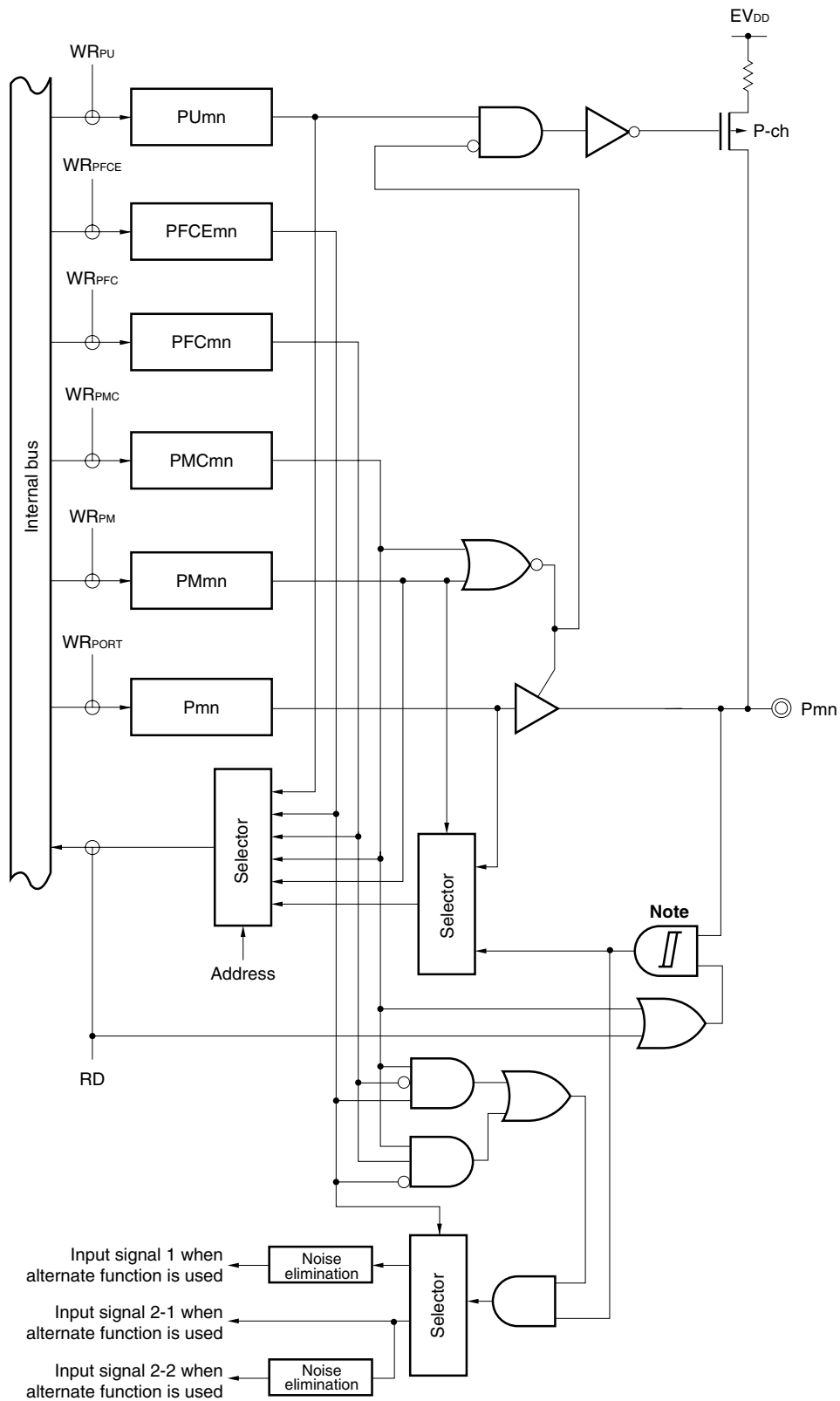
Figure 4-20. Block Diagram of Type U-7
