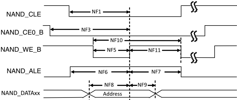
Figure 25. Address Latch cycle timing diagram
