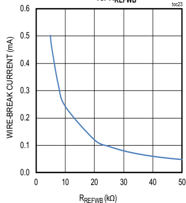
WIRE-BREAK CURRENT THRESHOLD vs. R_{REFWB}
