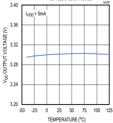
LDO OUTPUT VOLTAGE vs. TEMPERATURE
