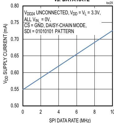
V_{DD} SUPPLY CURRENT vs. DATA RATE
