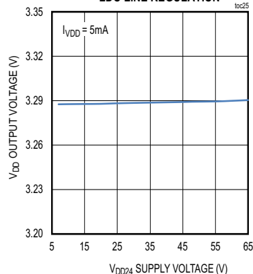
LDO LINE REGULATION
