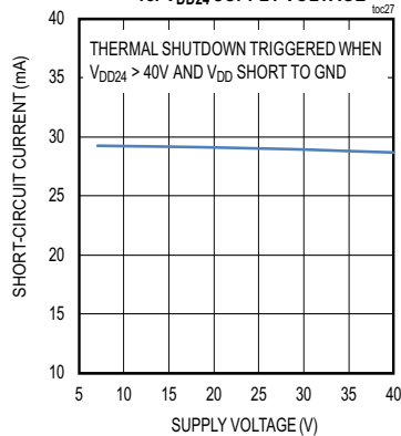
LDO SHORT-CIRCUIT CURRENT vs. V_{DD24} SUPPLY VOLTAGE
