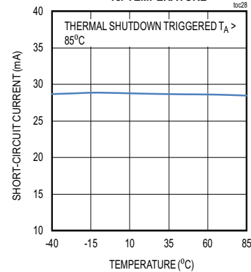
LDO SHORT-CIRCUIT CURRENT vs. TEMPERATURE
