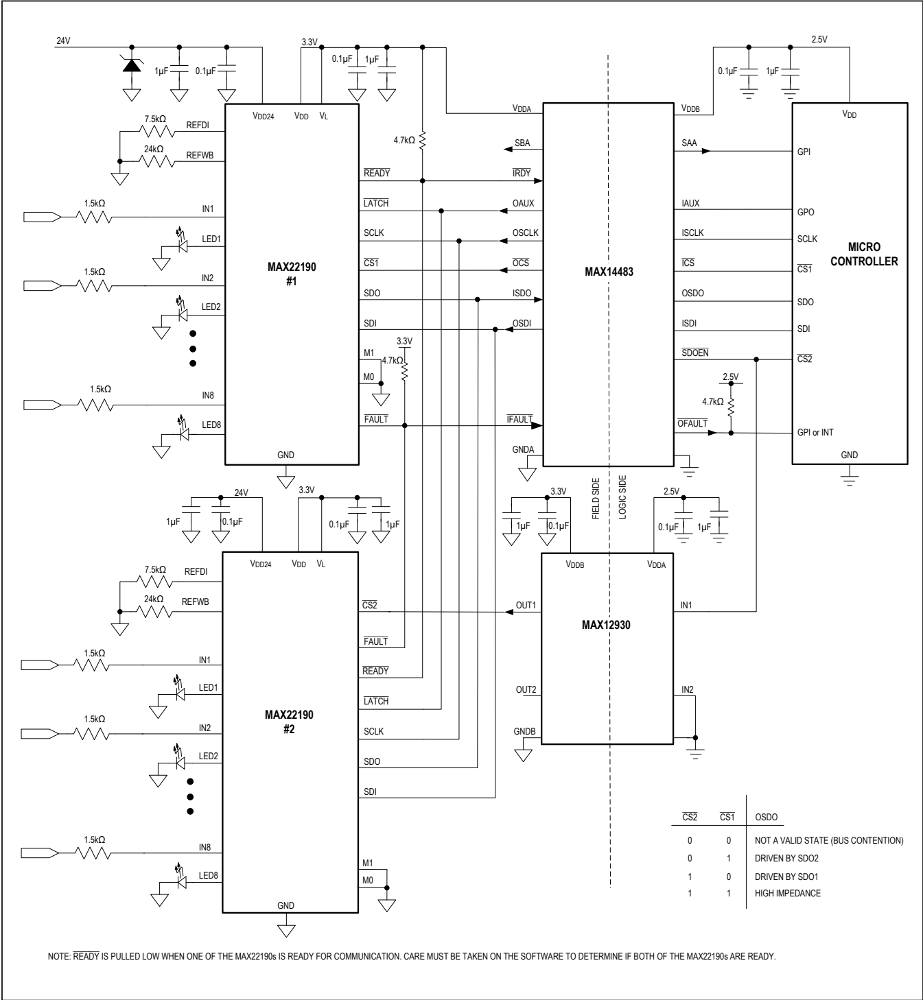
Figure 10. 16-Channel Type 1/3 Digital Input, Independent Slave SPI (Separate \overline{\text{CS}} for Each SPI Slave)
