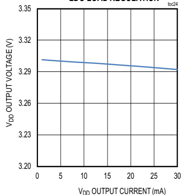
LDO LOAD REGULATION
