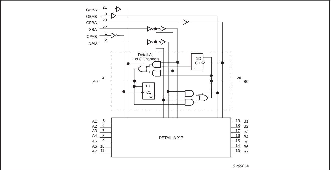
LOGIC DIAGRAM
