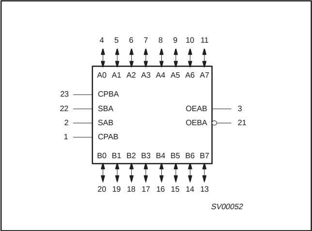
LOGIC SYMBOL
