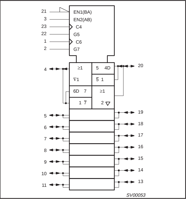
LOGIC SYMBOL (IEEE/IEC)
