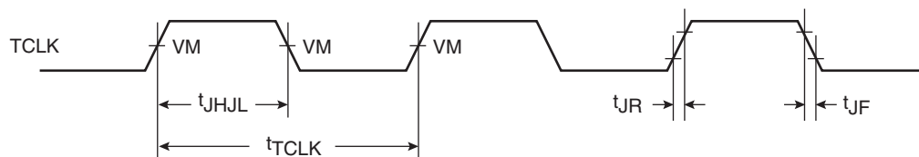
Figure 7-12. JTAG Clock Input Timing Diagram
