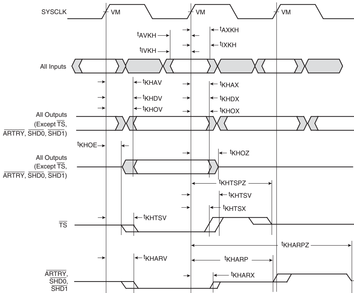
Figure 7-3. Input/Output Timing Diagram
