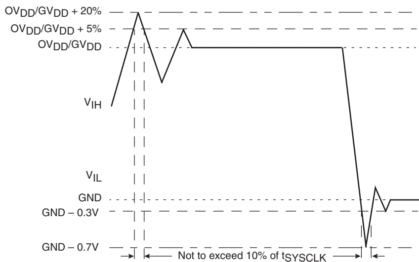
Figure 6-1. Overshoot/Undershoot Voltage
