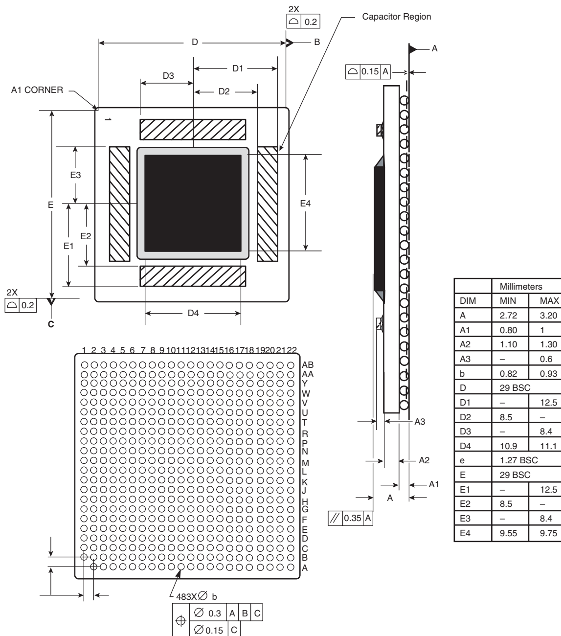
Figure 9-1. Mechanical Dimensions and Bottom Surface Nomenclature for the PC7457, 483 CBGA Package
