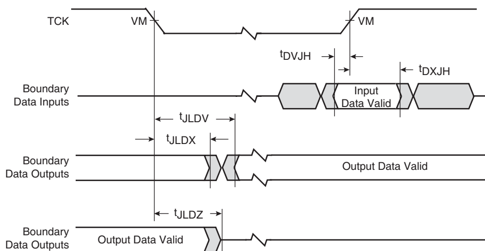
Figure 7-14. Boundary-scan Timing Diagram
