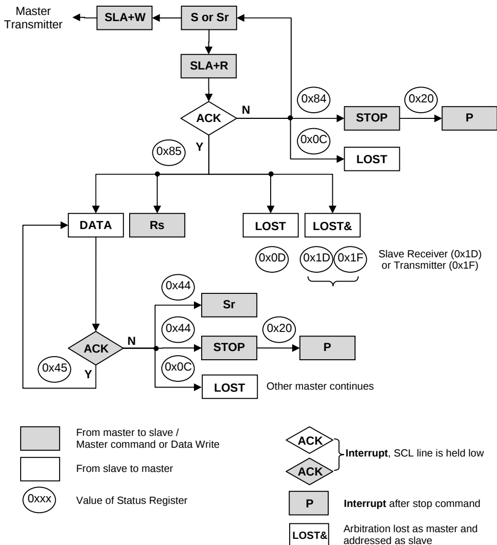
Figure 11-59 Formats and States in the Master Receiver Mode
