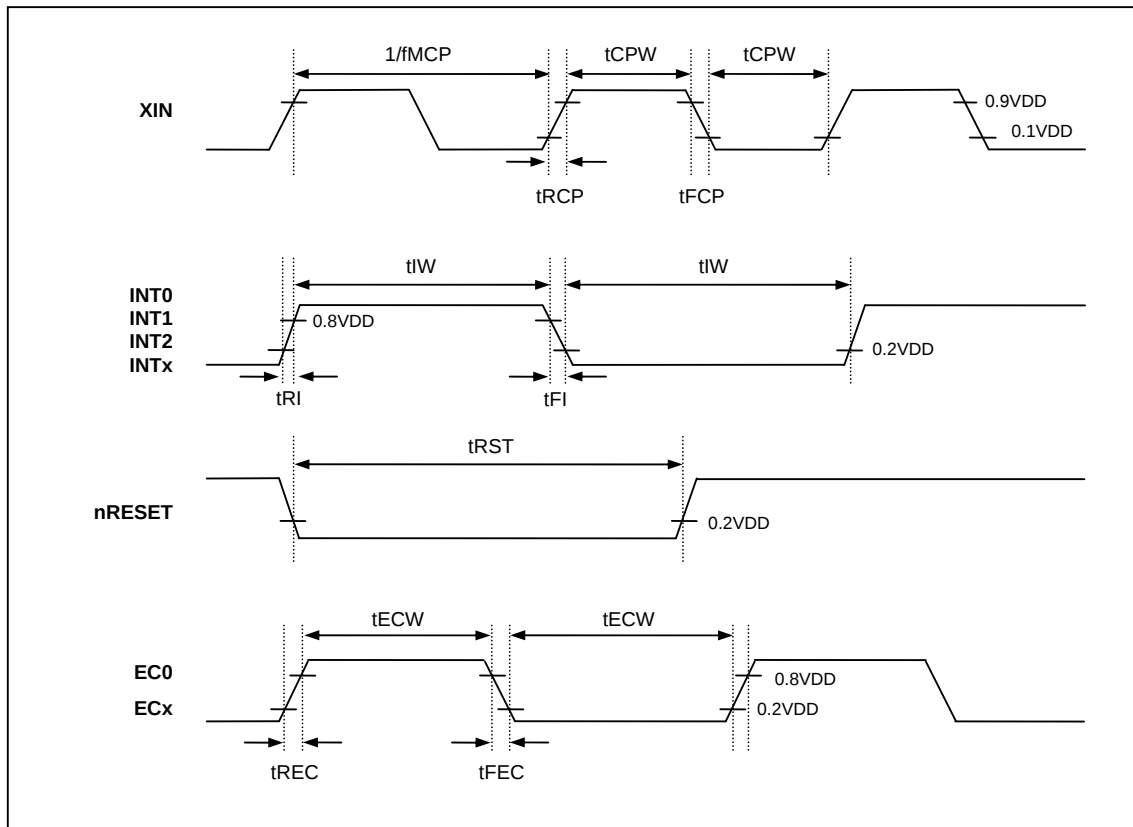
Figure 7-1 AC Timing
