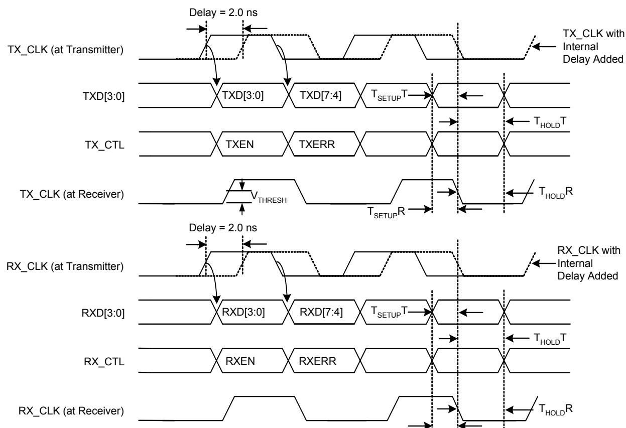
Figure 22. RGMII Compensated Timing
