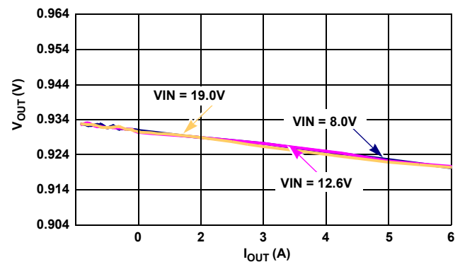
FIGURE 9. 1-PHASE DE MODE LOAD LINE, \text{PSI}_I = LOW, \text{VID} = 0.9V, \text{OFFSET} = 33mV
