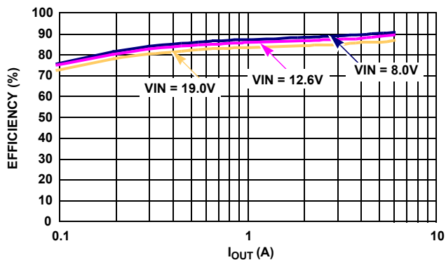
FIGURE 8. EFFICIENCY OF 1-PHASE DE MODE, \text{PSI}_I = LOW, DCM MODE, \text{VID} = 0.9V, \text{OFFSET} = 33mV
