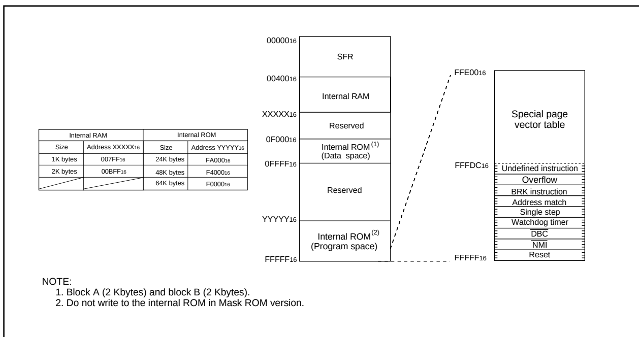
Figure 3.1 Memory Map
