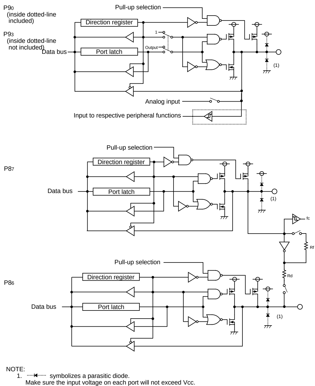
Figure 16.4. I/O Ports (4)
