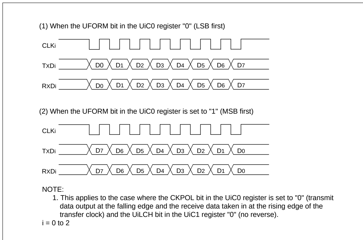
Figure 13.1.1.3.1 Transfer format
