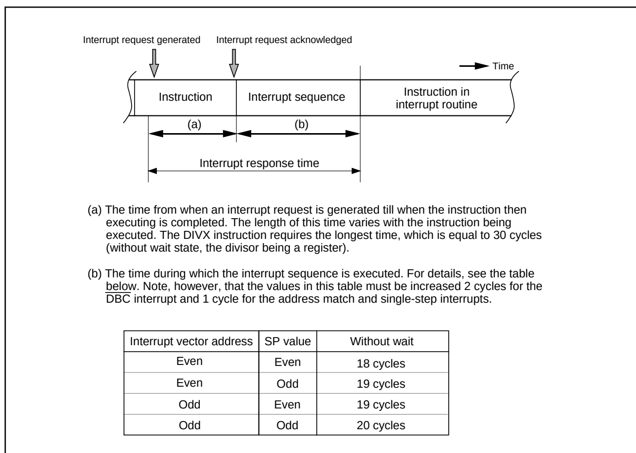
Figure 9.4.1.1. Interrupt response time
