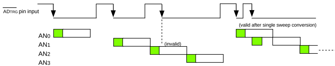
Figure 14.1.8.1 Operation Example in Delayed Trigger Mode1
