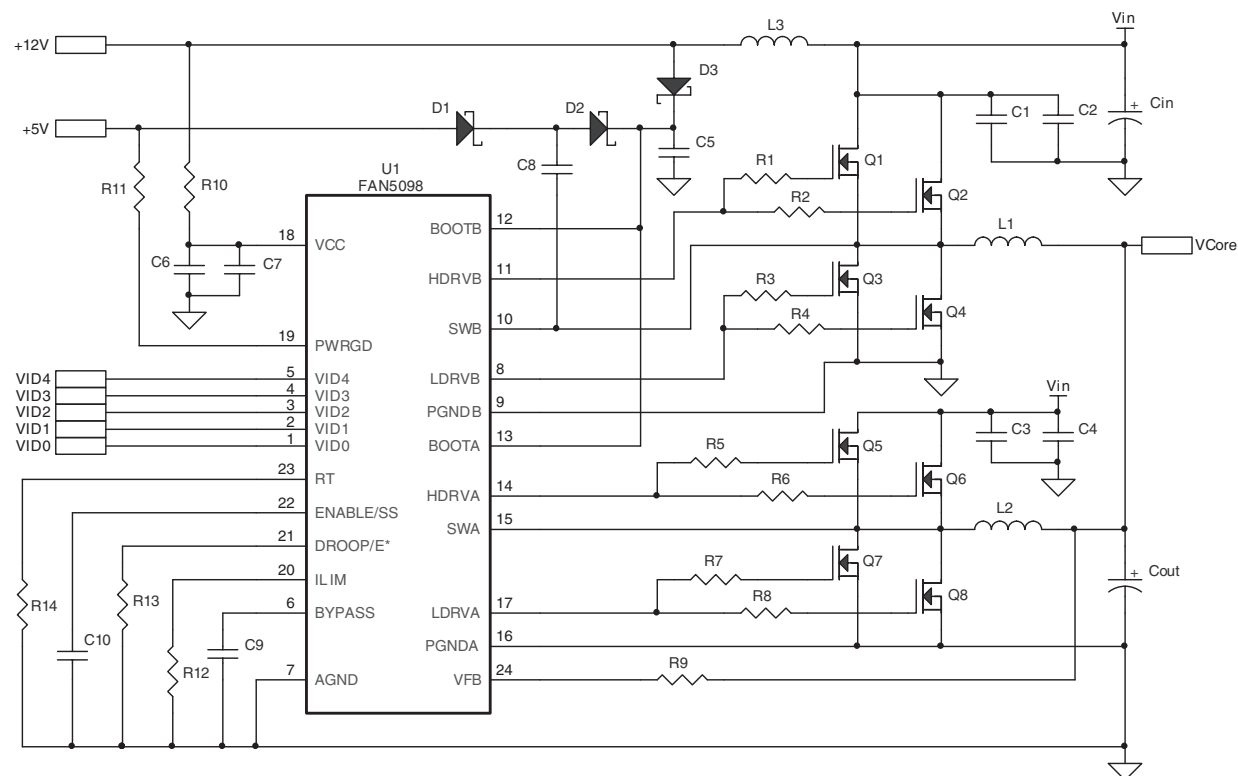
Figure 2. Application Circuit for 56A AMD® Hammer™ Desktop Application
