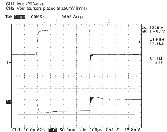
LOAD TRANSIENT, 12-52A
