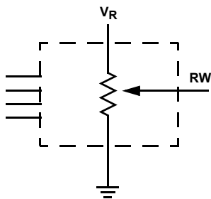
FIGURE 11. THREE TERMINAL POTENTIOMETER; VARIABLE VOLTAGE DIVIDER
