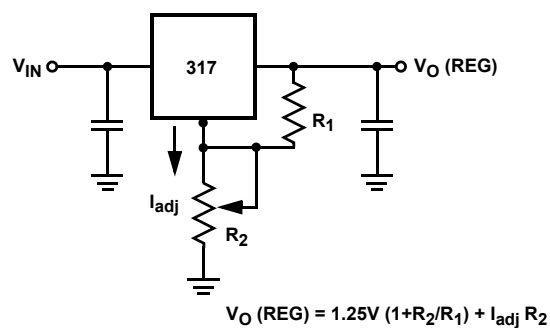
FIGURE 14. VOLTAGE REGULATOR
