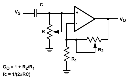
FIGURE 18. FILTER
