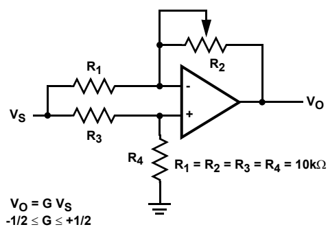
FIGURE 17. ATTENUATOR
