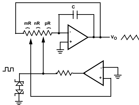
FIGURE 24. FUNCTION GENERATOR
