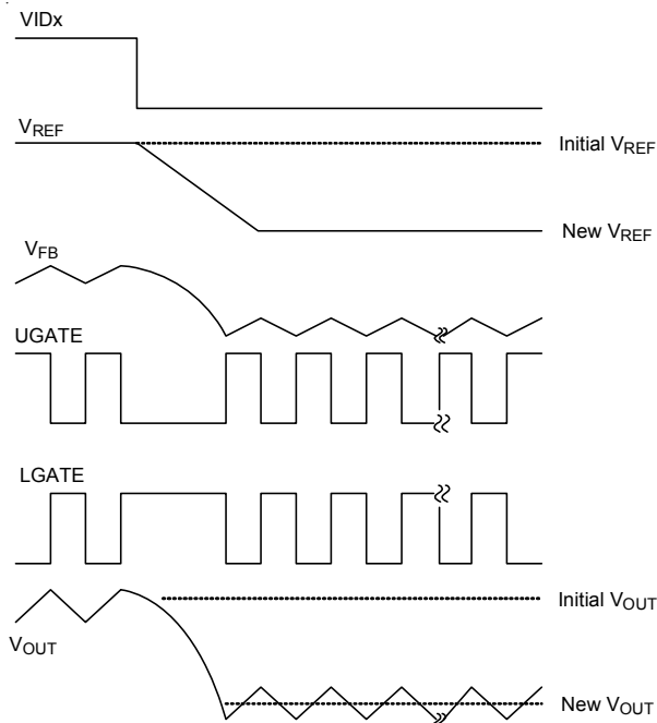
Figure 2. Down Transition of Output Voltage
