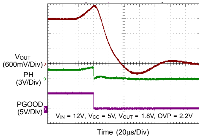
Over-Voltage Protection
