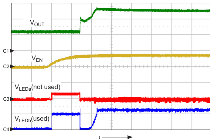
Figure 3. LED detect circuit operation for an LED pin that is not being used; shows V_{OUT} (ch1, 10 V/div.), V_{EN} (ch2, 5 V/div.), an unused LEDx with a 2.4 k \Omega resistor from this pin to GND, V_{LEDa} (ch3, 500 mV/div.), and a used LEDx, V_{LEDb} (ch4, 500 mV/div.), t = 2 ms/div.
