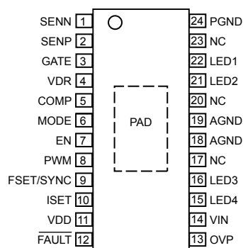
LP Package
