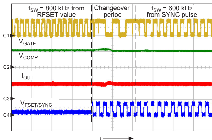
Figure 13. Synchronization feature with 200 kHz difference between R FSET and external clock signal. The synchronization frequency is 600 kHz, and the resistor preset frequency is 800 kHz. Note that there is very little disturbance in the LED current at the time of changeover; shows V GATE (ch1, 5 V/div.), V COMP (ch2, 1 V/div.), I OUT (ch3, 1 A/div.), and V FSET/SYNC (ch4, 5 V/div.), t = 5 \mu s/div.
