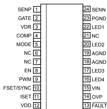
LB Package
