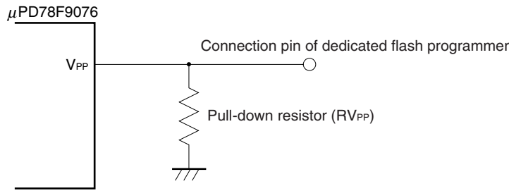
Figure 13-4 V PP Pin Connection Example
