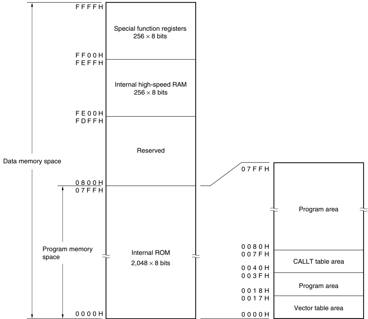
Figure 3-1. Memory Map ( \mu PD789071)
